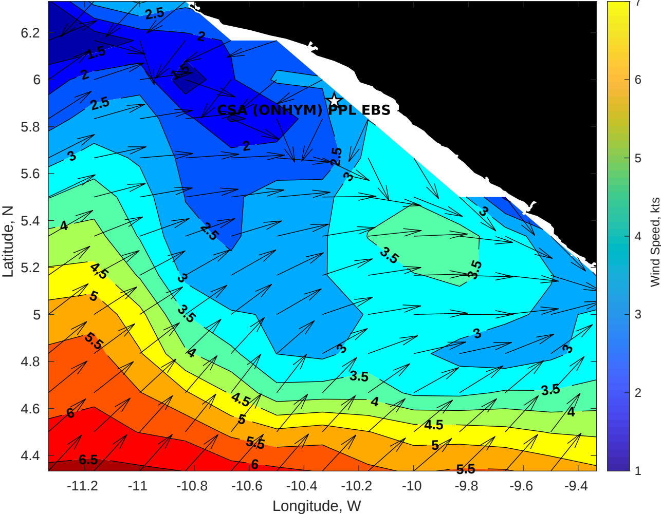
GFS Winds (kts) for CSA (ONHYM) PPL EBS - Liberia at 08-Dec-2025 09:00:00
