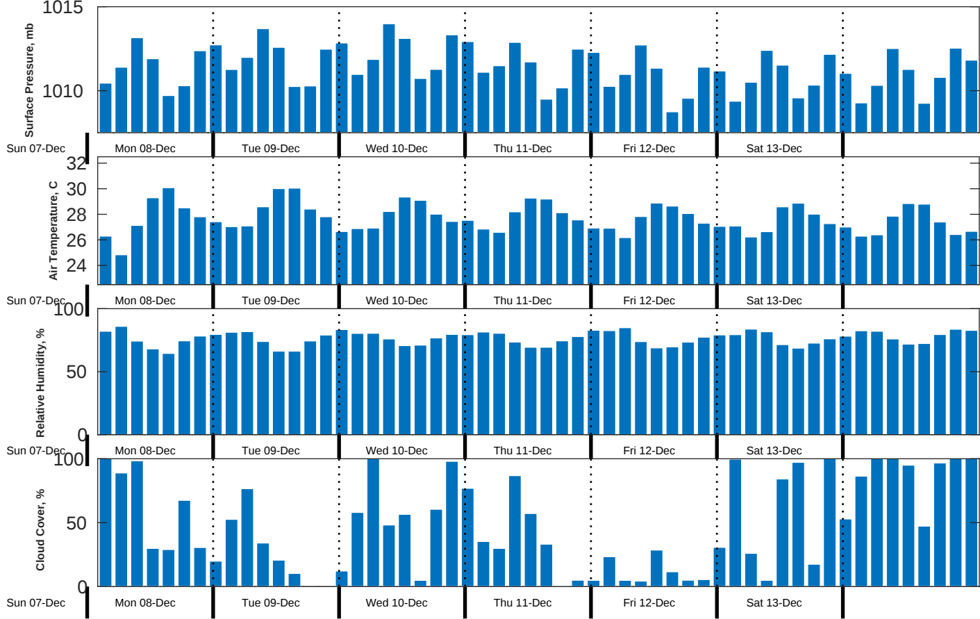
Met Forecast for CSA (ONHYM) PPL EBS - Liberia from 08-Dec-2025 00:00:00 to 15-Dec-2025 00:00:00
