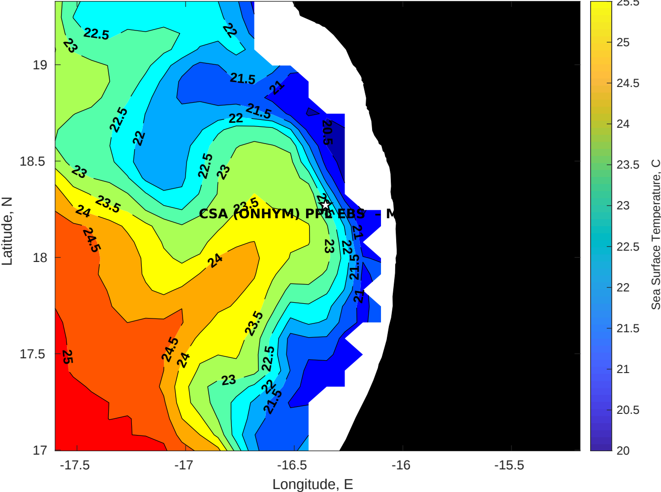
SST for CSA (ONHYM) PPL EBS - Mauritania at 07-Dec-2025 00:00:00
