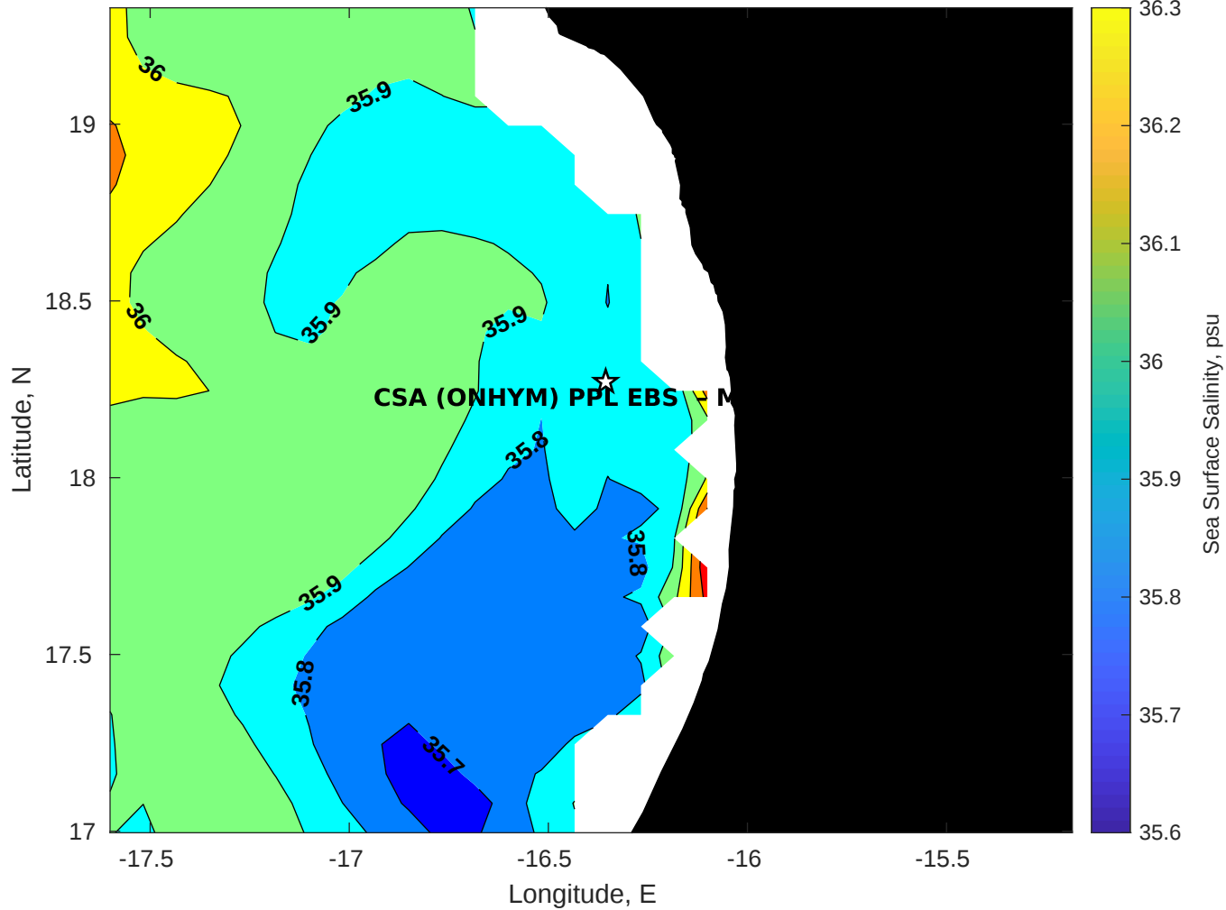
Surface Salinity for CSA (ONHYM) PPL EBS - Mauritania at 07-Dec-2025 00:00:00
