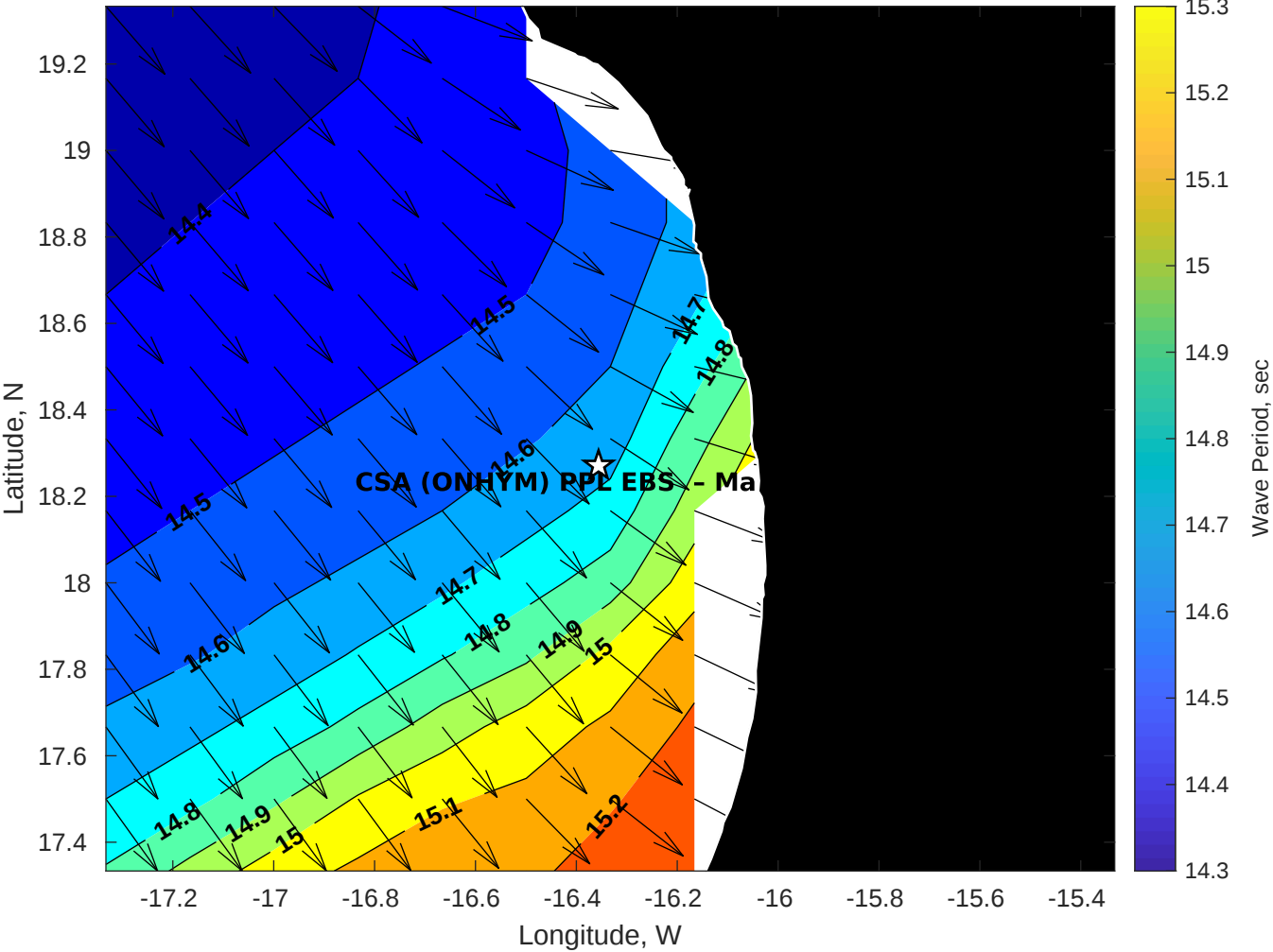
GFS Wave Period (sec) for CSA (ONHYM) PPL EBS - Mauritania at 08-Dec-2025 09:00:00
