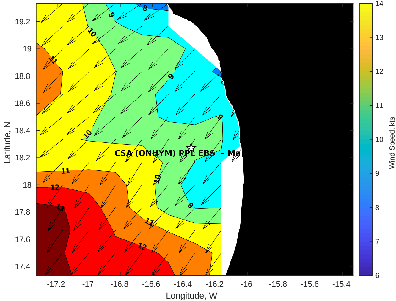
GFS Winds (kts) for CSA (ONHYM) PPL EBS - Mauritania at 08-Dec-2025 09:00:00
