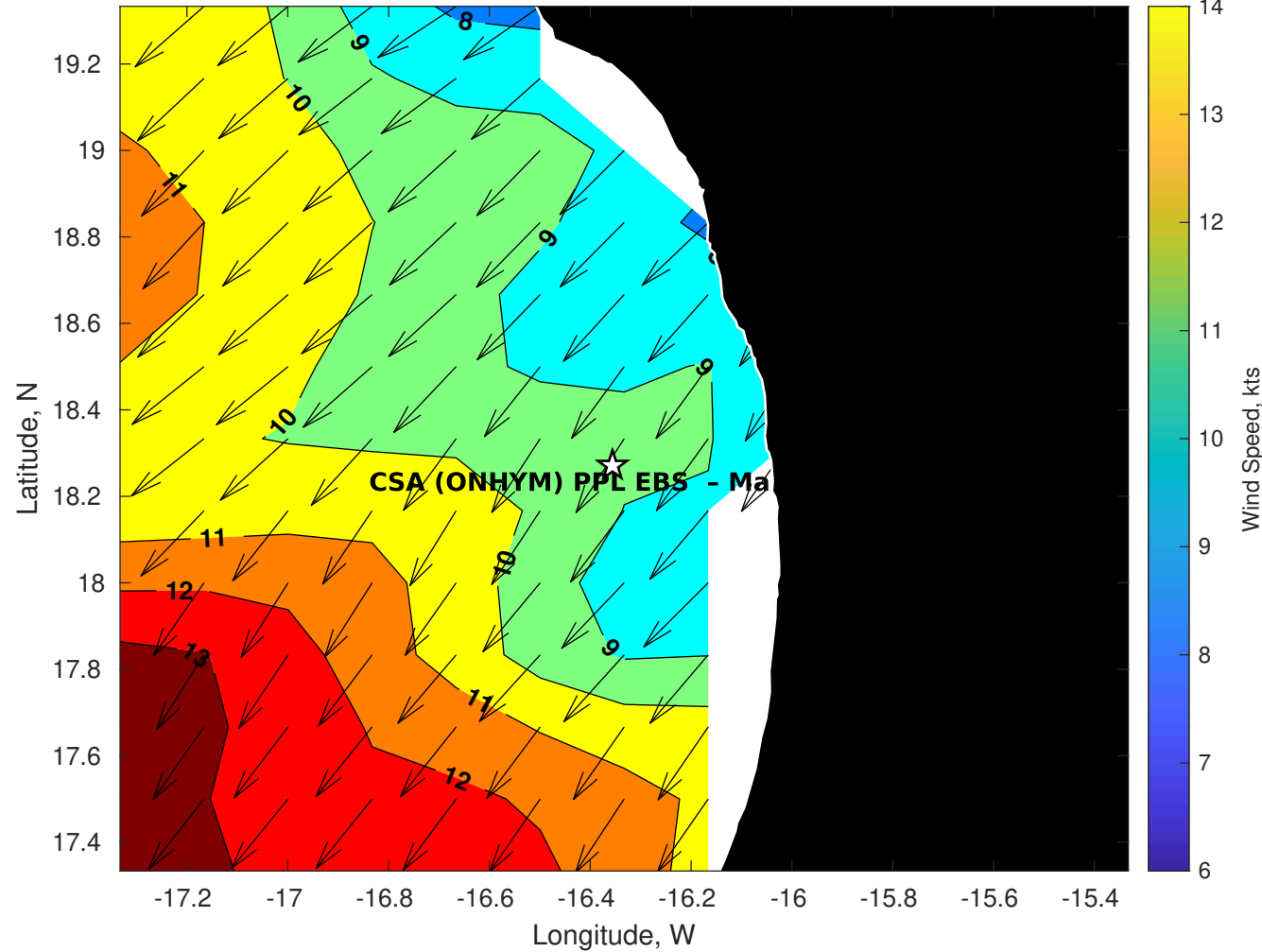
GFS Winds (kts) for CSA (ONHYM) PPL EBS - Mauritania at 08-Dec-2025 09:00:00
