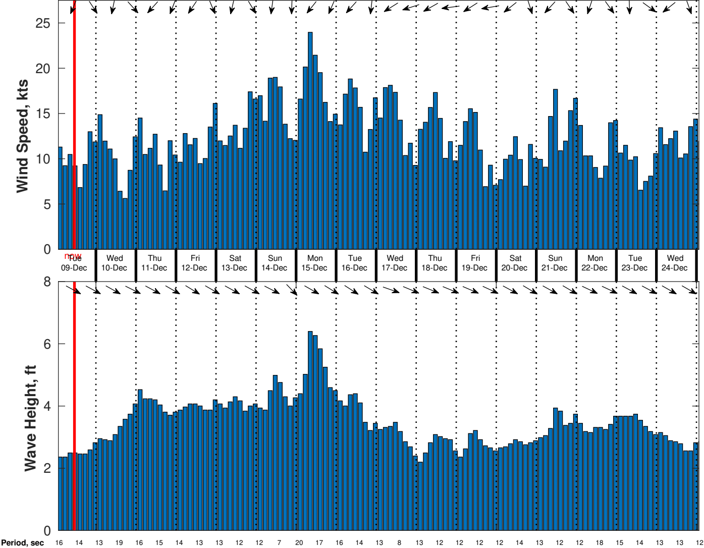
Wind & Wave Forecast for CSA (ONHYM) PPL EBS - Mauritania from 08-Dec-2025 01:00:00 to 24-Dec-2025 01:00:00
