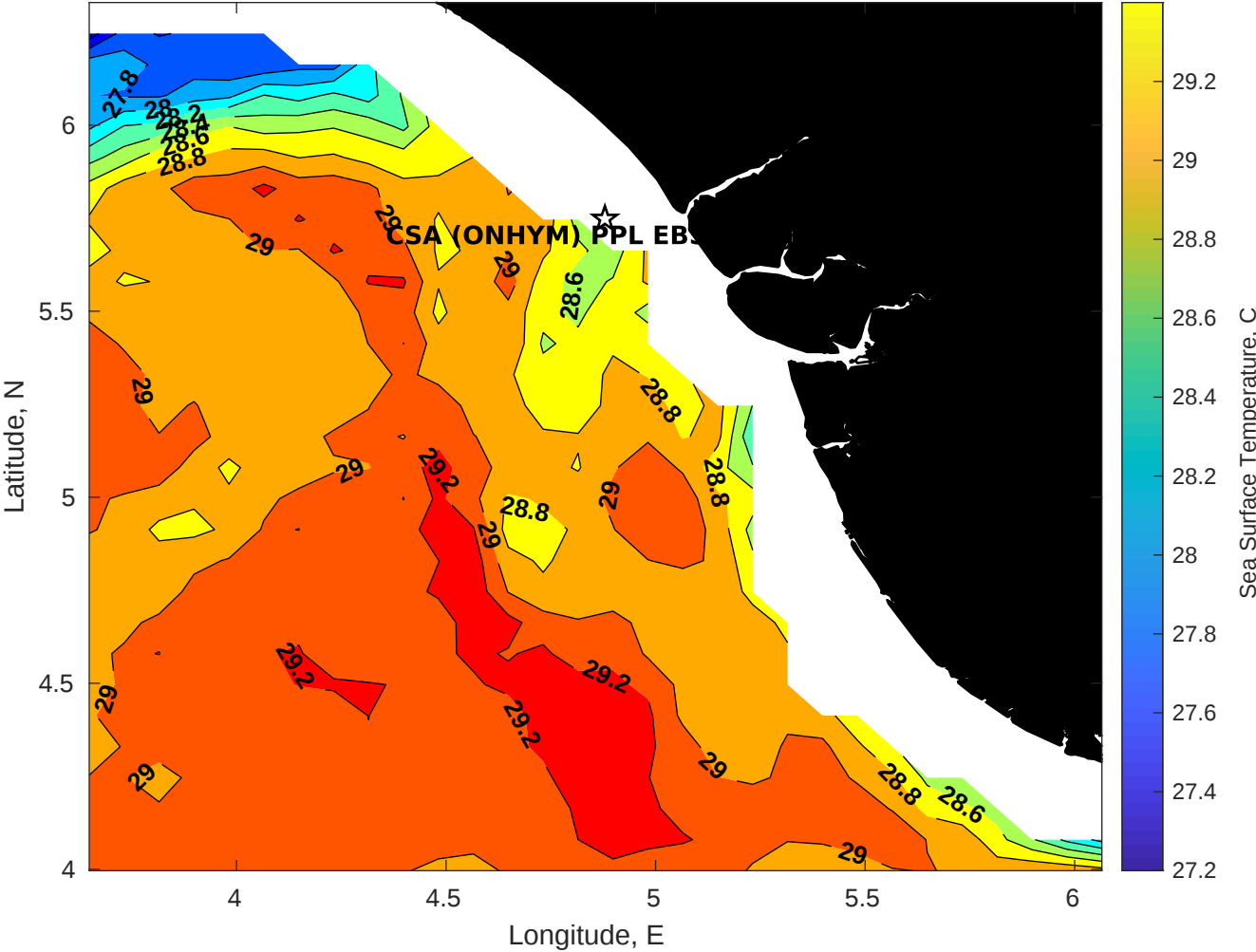
SST for CSA (ONHYM) PPL EBS - Nigeria at 07-Dec-2025 00:00:00
