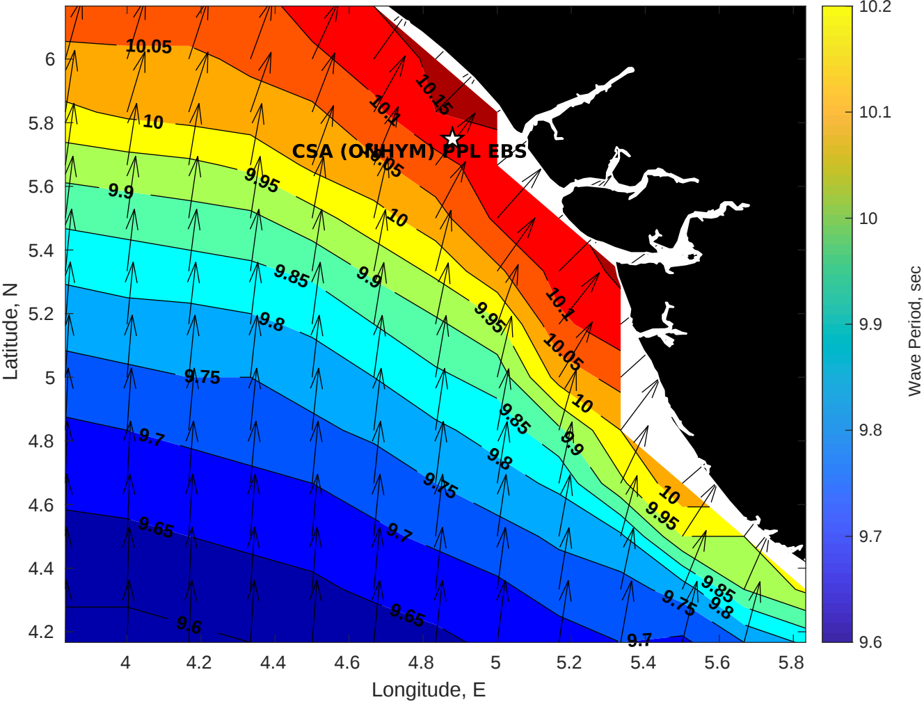
GFS Wave Period (sec) for CSA (ONHYM) PPL EBS - Nigeria at 08-Dec-2025 09:00:00
