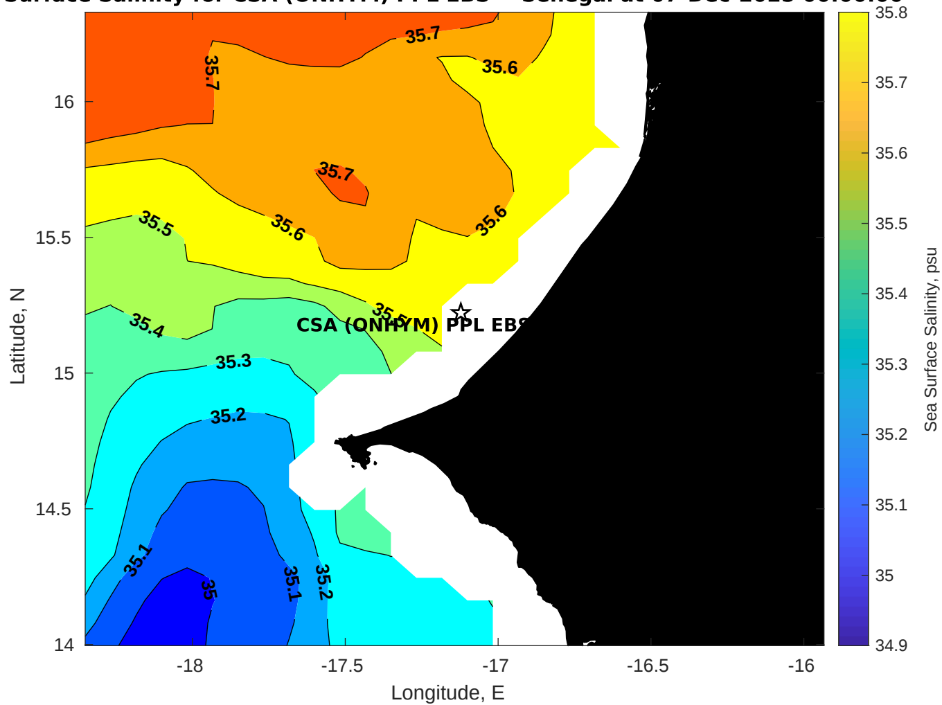
Surface Salinity for CSA (ONHYM) PPL EBS - Senegal at 07-Dec-2025 00:00:00
