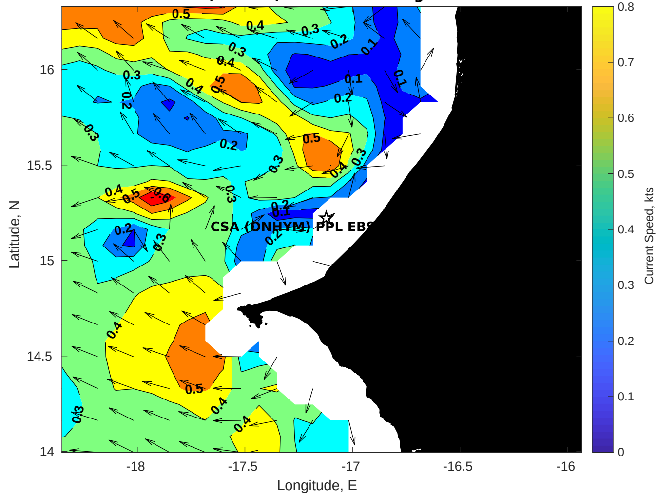
Surface Currents for CSA (ONHYM) PPL EBS - Senegal at 07-Dec-2025 00:00:00
