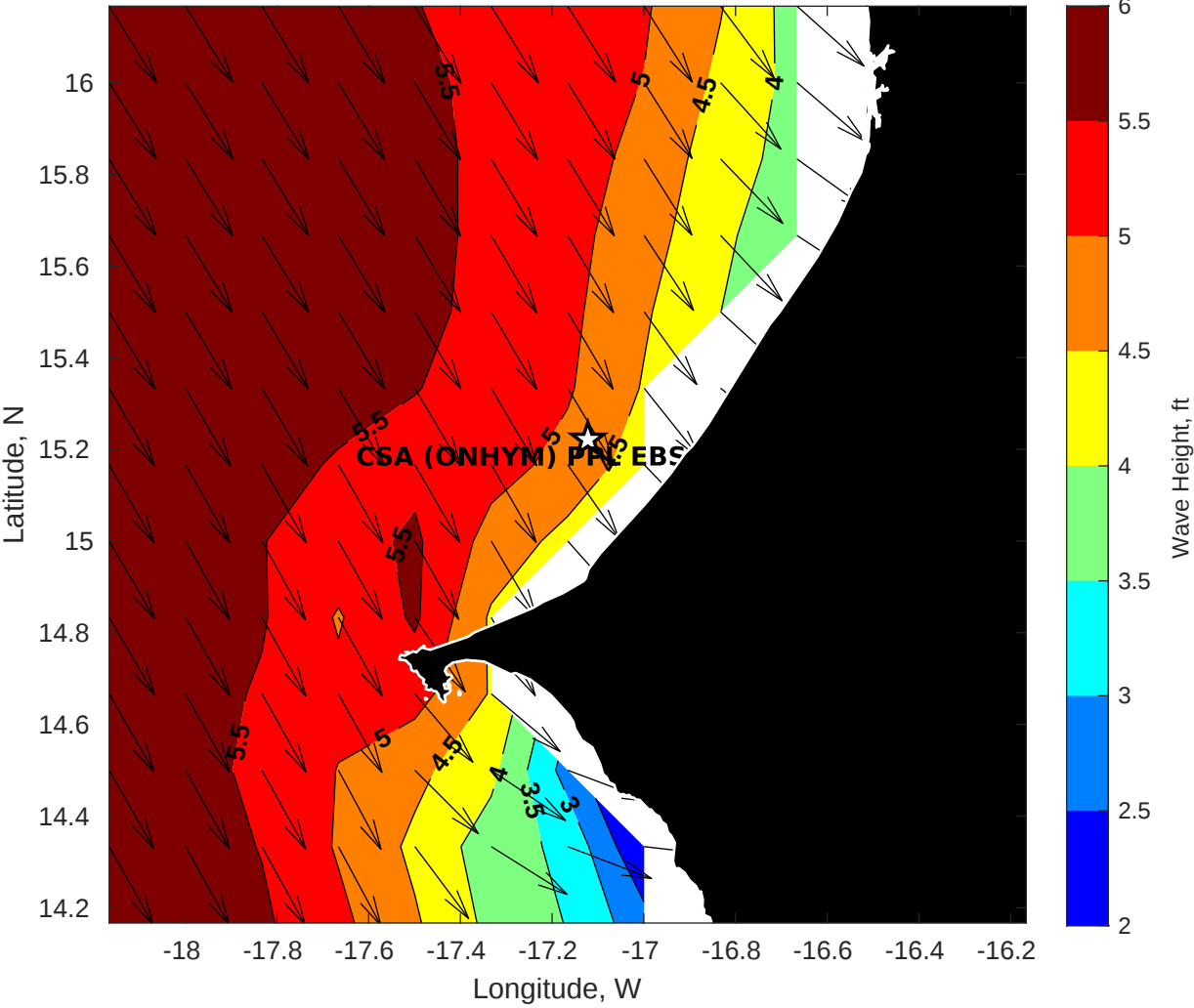
GFS Wave Height (ft) for CSA (ONHYM) PPL EBS - Senegal at 08-Dec-2025 09:00:00
