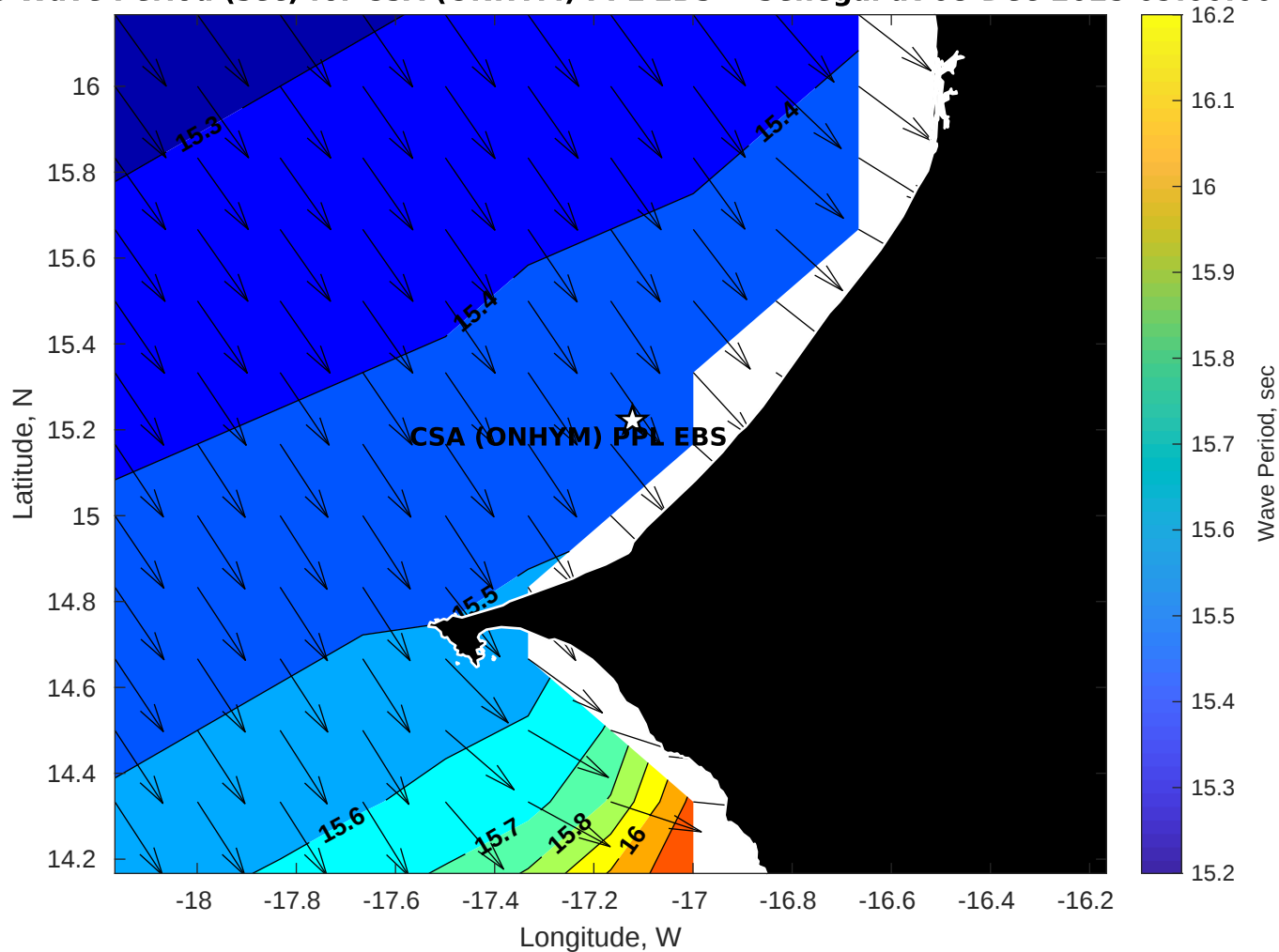
GFS Wave Period (sec) for CSA (ONHYM) PPL EBS - Senegal at 08-Dec-2025 09:00:00
