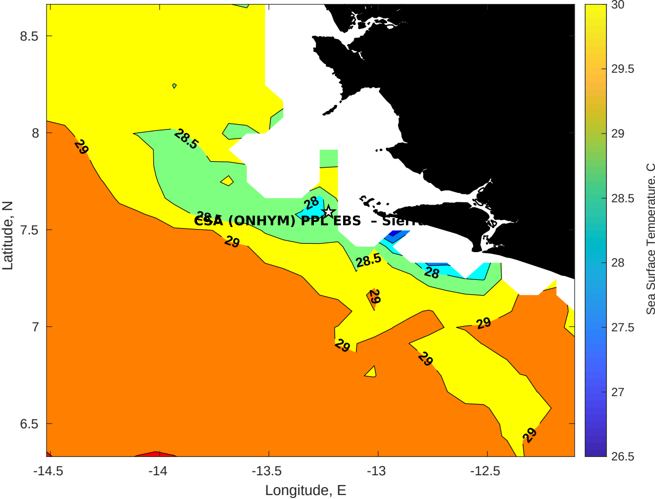
SST for CSA (ONHYM) PPL EBS - Sierra Leone at 07-Dec-2025 00:00:00
