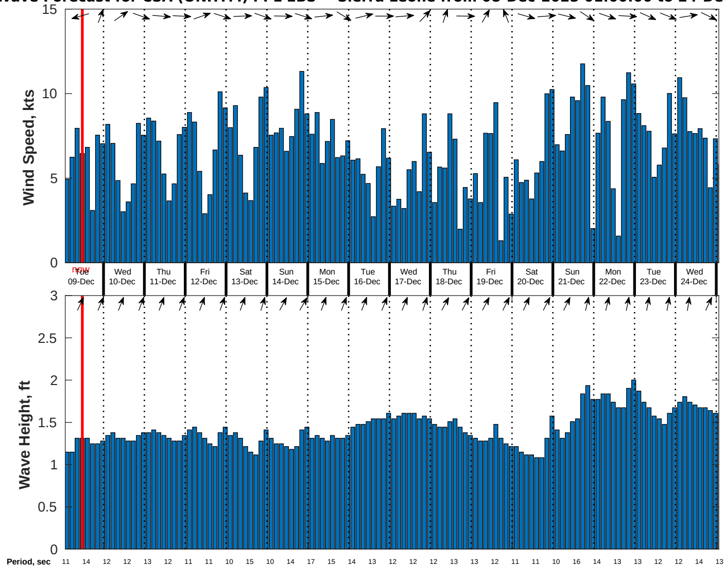
Wind & Wave Forecast for CSA (ONHYM) PPL EBS - Sierra Leone from 08-Dec-2025 01:00:00 to 24-Dec-2025 01:00:00
