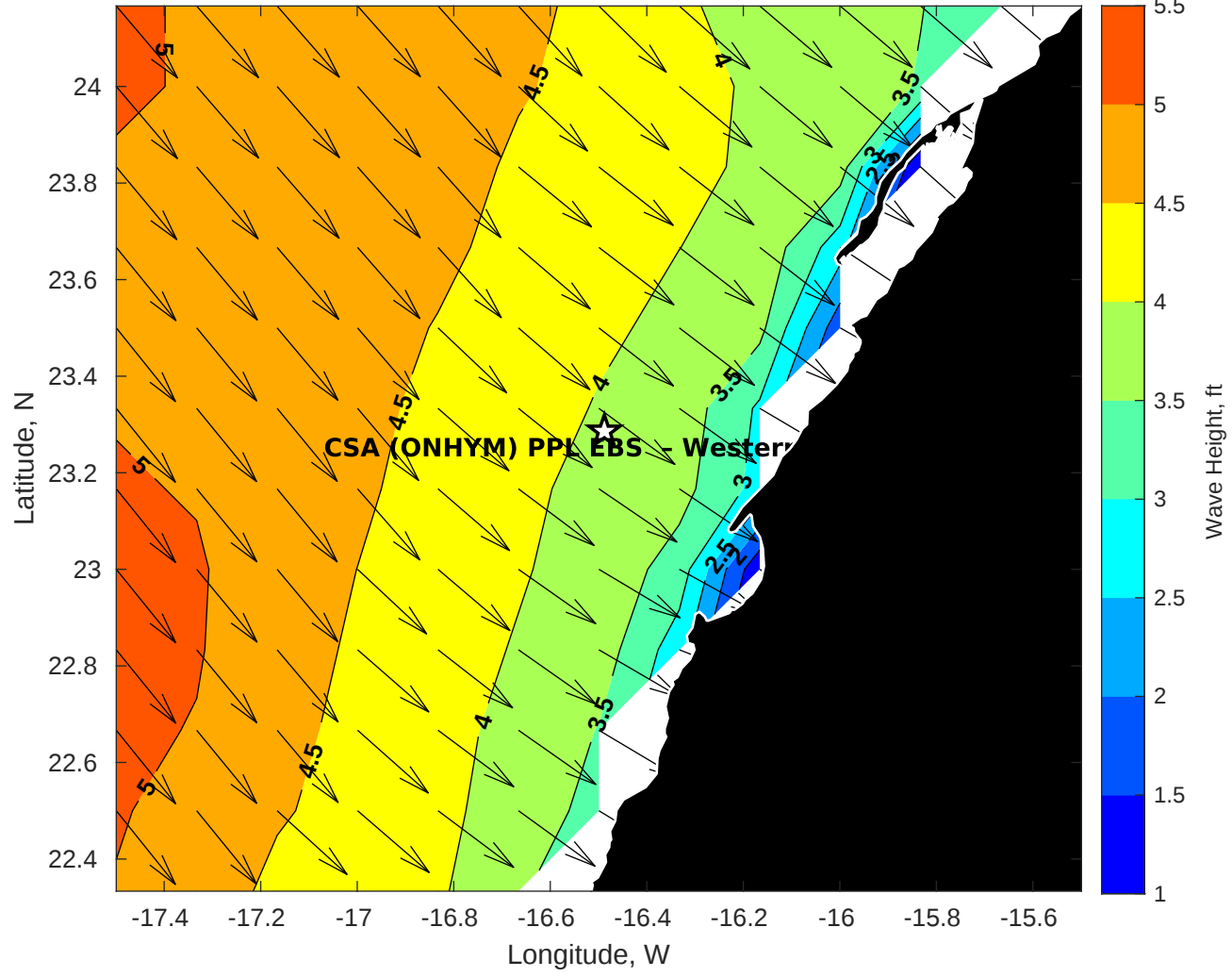
GFS Wave Height (ft) for CSA (ONHYM) PPL EBS - Western Sahara at 08-Dec-2025 09:00:00
