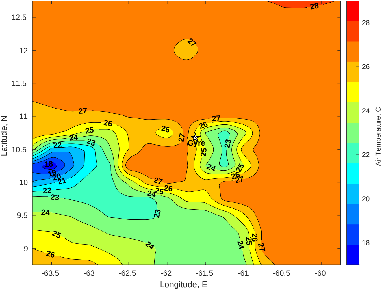
Air Temperature (C) for Gyre at 08-Dec-2025
