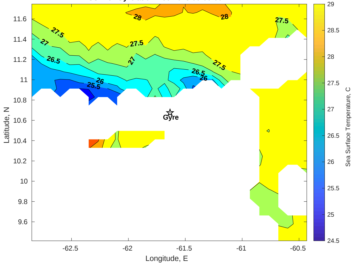
SST for Gyre at 07-Dec-2025 00:00:00
