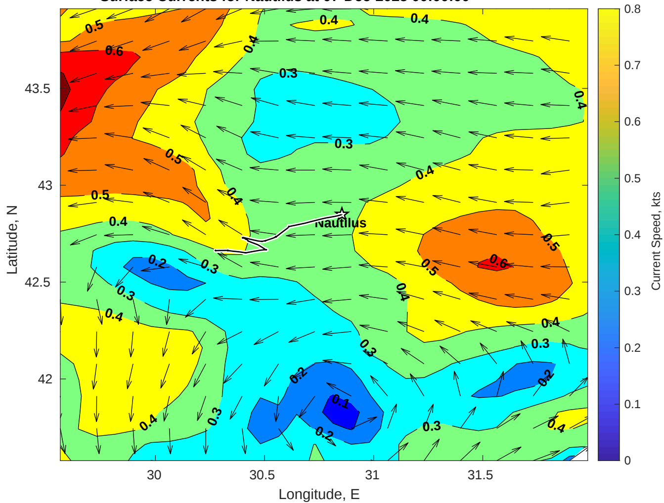
Surface Currents for Nautilus at 07-Dec-2025 00:00:00
