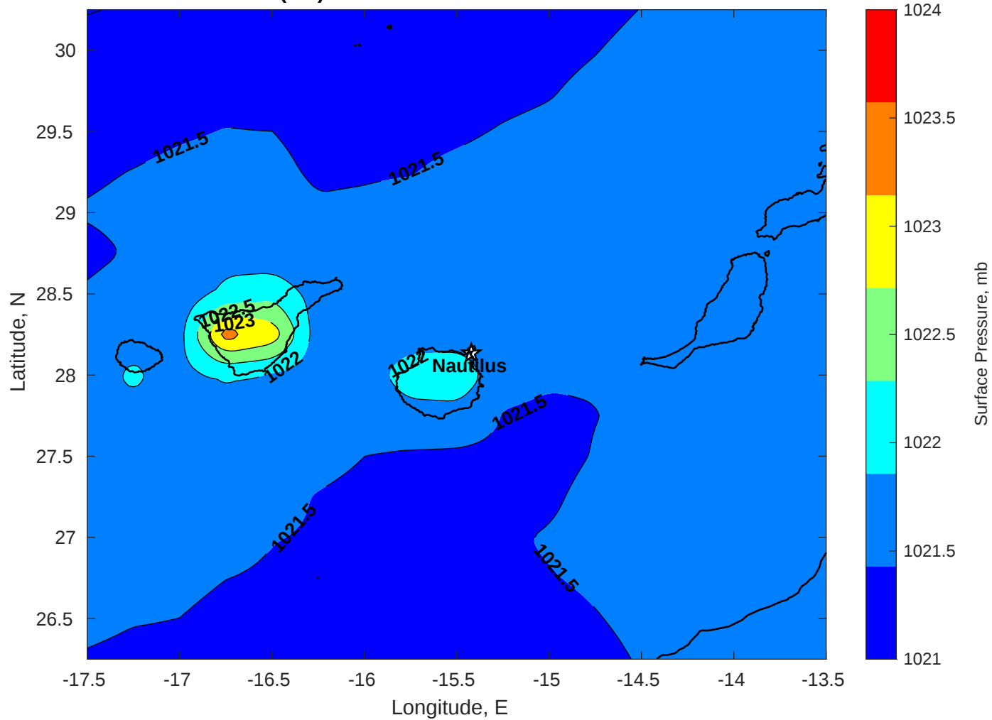
Surface Pressure (mb) for Nautilus at 09-Dec-2025 00:00:00
