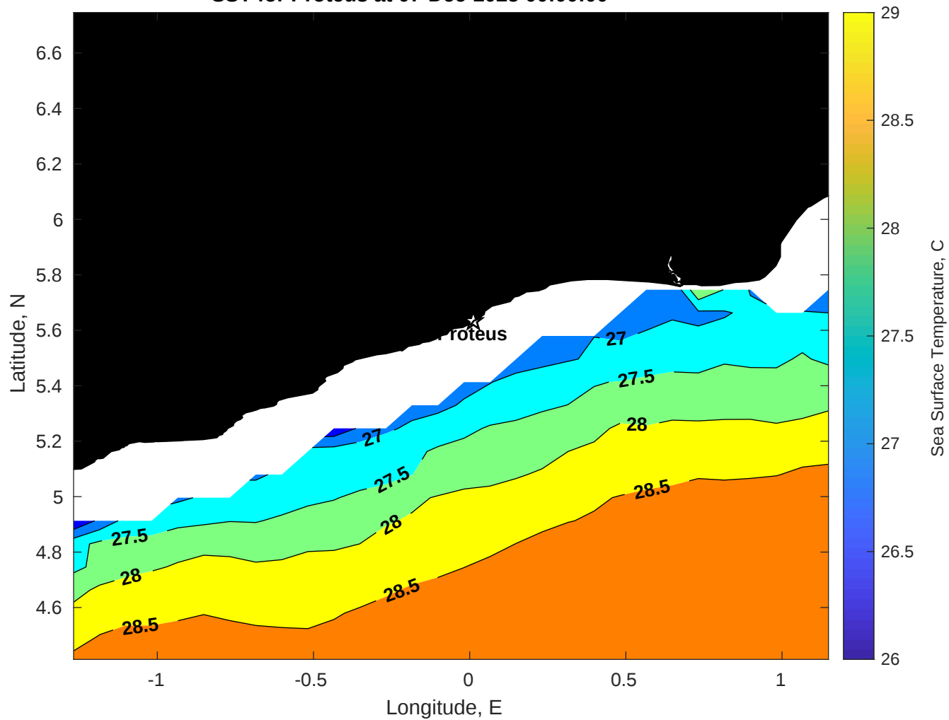
SST for Proteus at 07-Dec-2025 00:00:00
