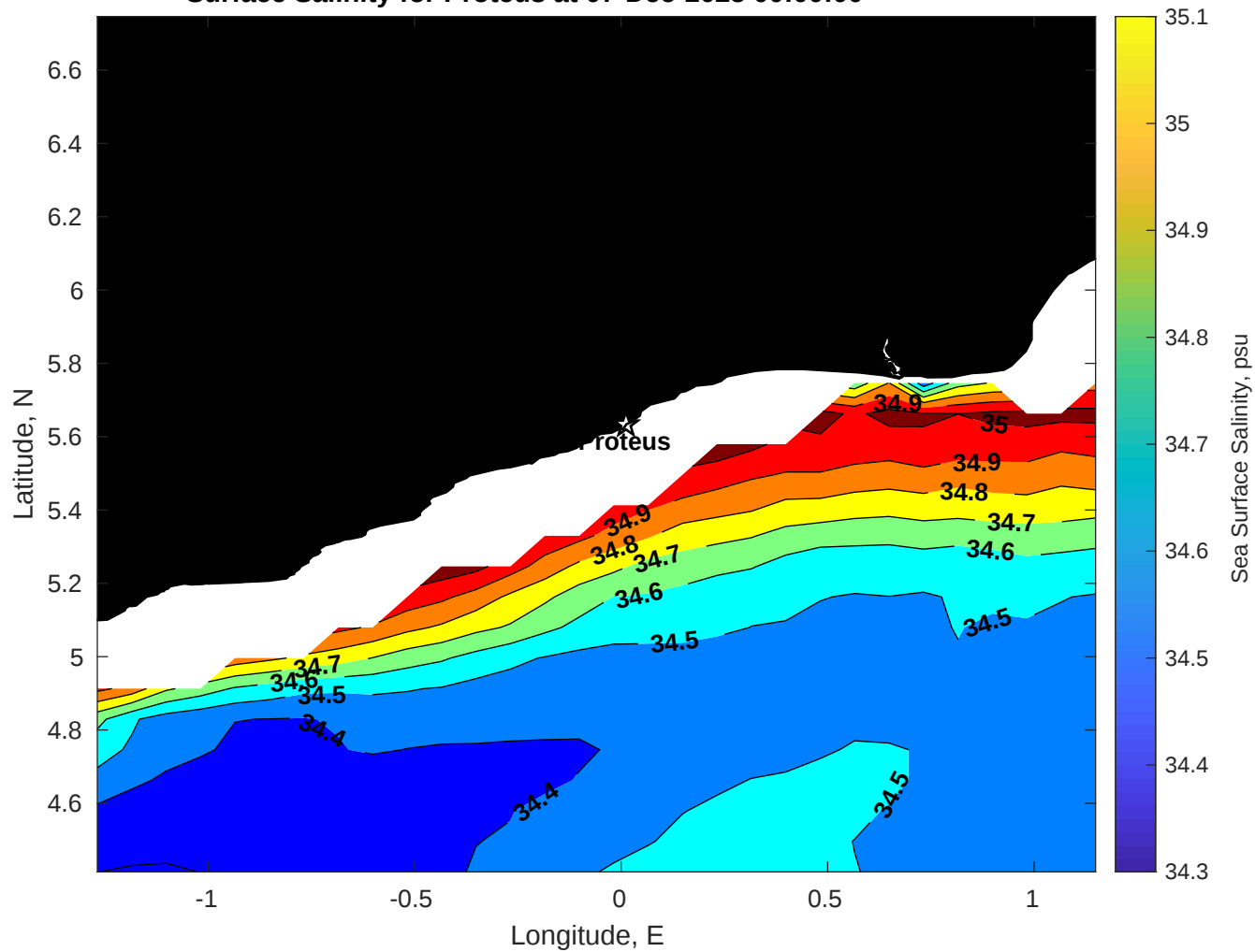
Surface Salinity for Proteus at 07-Dec-2025 00:00:00
