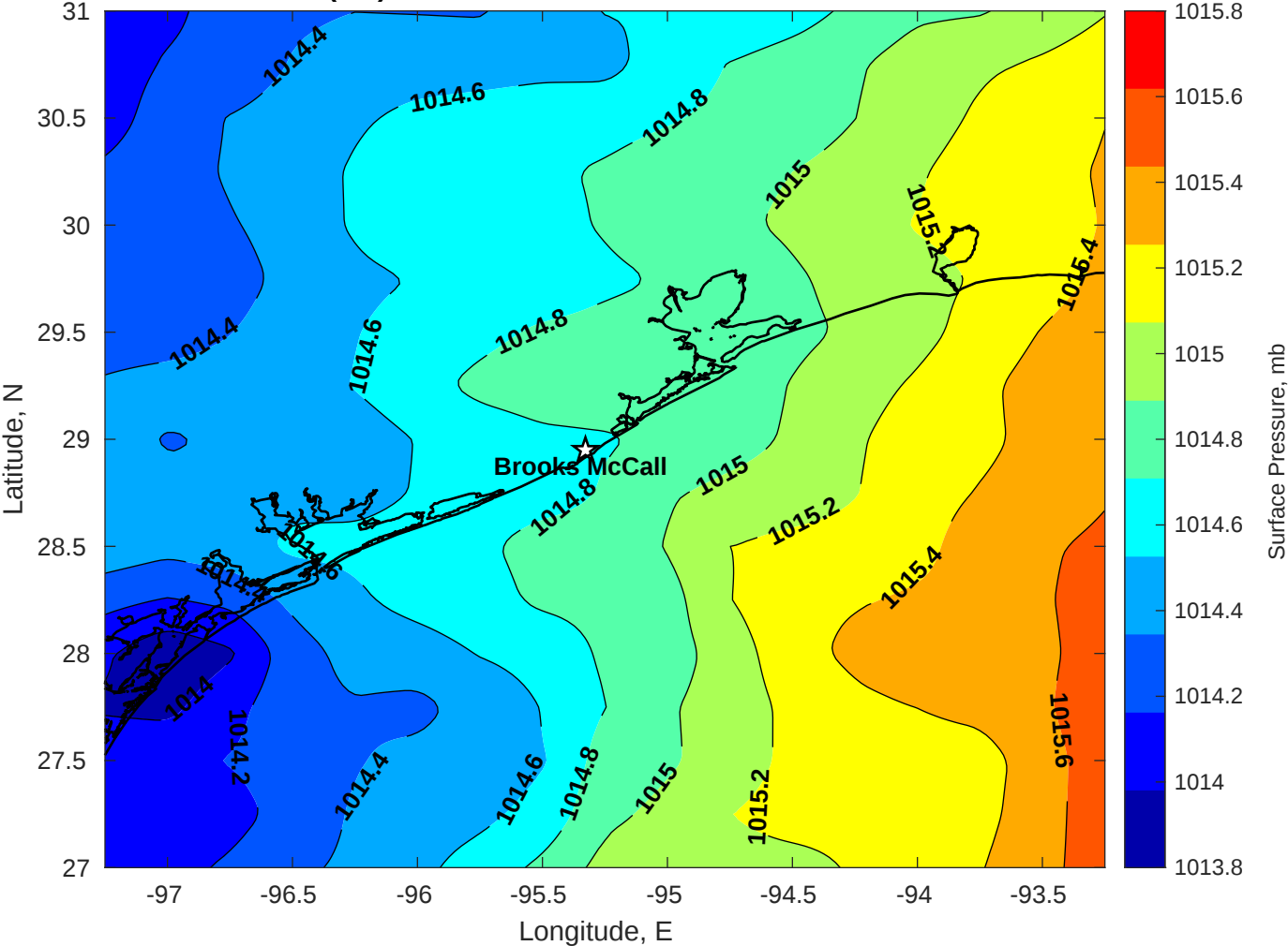
Surface Pressure (mb) for Brooks McCall at 10-Dec-2025 12:00:00
