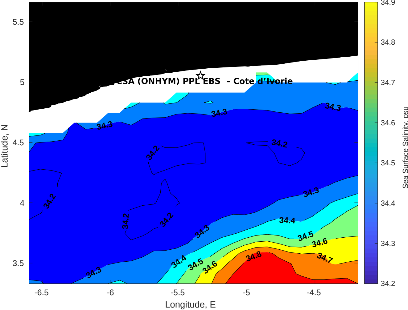
Surface Salinity for CSA (ONHYM) PPL EBS - Cote d'Ivoire at 08-Dec-2025 00:00:00
