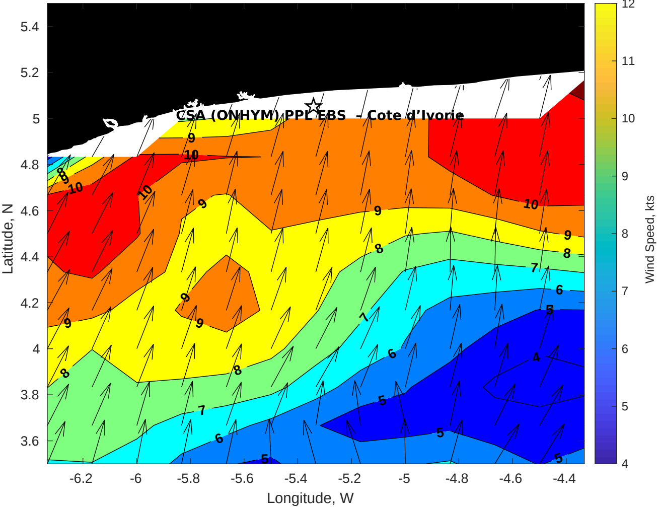
GFS Winds (kts) for CSA (ONHYM) PPL EBS - Cote d'Ivoire at 08-Dec-2025 21:00:00
