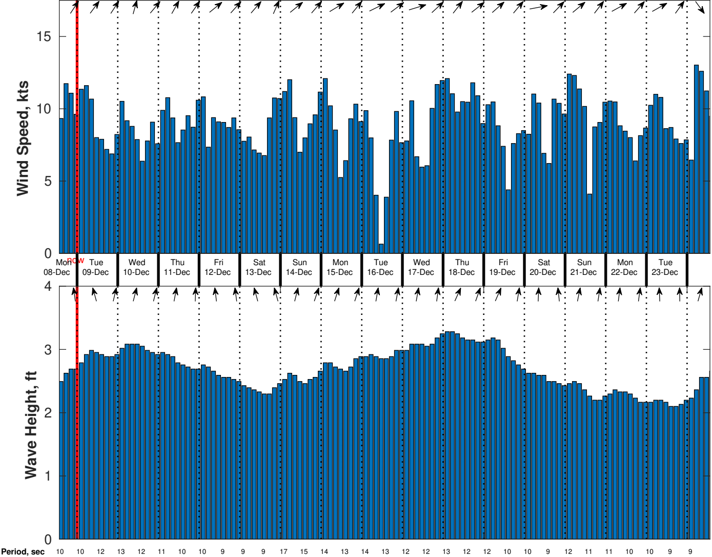
Wind & Wave Forecast for CSA (ONHYM) PPL EBS - Cote d'Ivoire from 08-Dec-2025 13:00:00 to 24-Dec-2025 13:00:00
