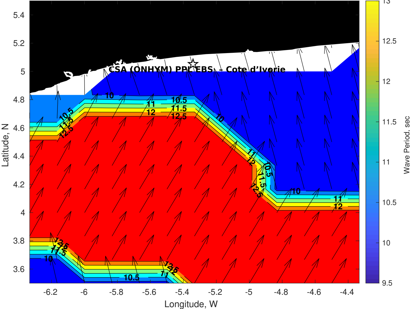
GFS Wave Period (sec) for CSA (ONHYM) PPL EBS - Cote d'Ivoire at 08-Dec-2025 21:00:00
