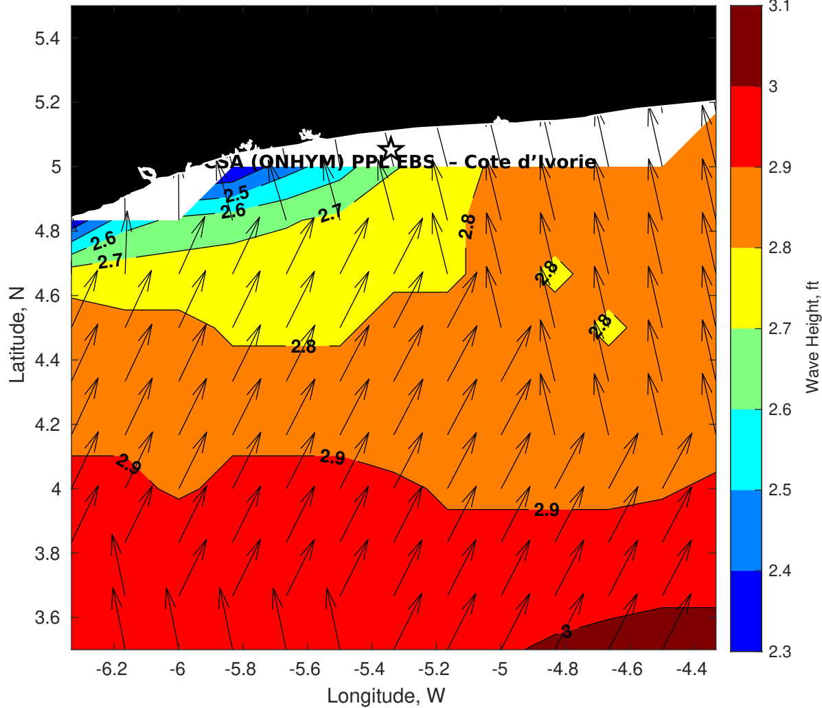
GFS Wave Height (ft) for CSA (ONHYM) PPL EBS - Cote d'Ivoire at 08-Dec-2025 21:00:00
