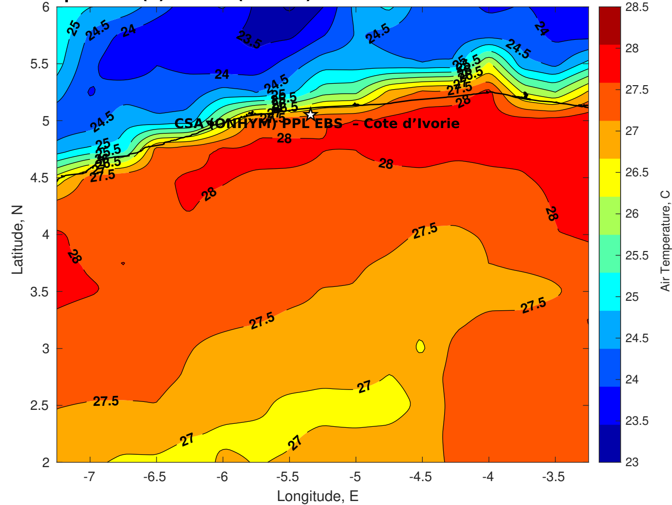
Air Temperature (C) for CSA (ONHYM) PPL EBS - Cote d'Ivoire at 09-Dec-2025
