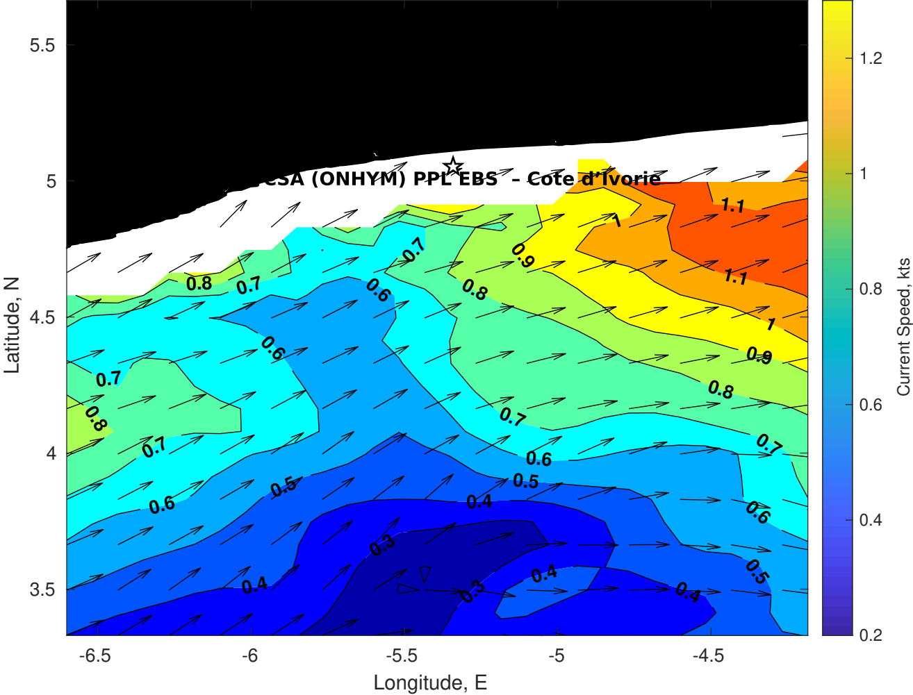
Surface Currents for CSA (ONHYM) PPL EBS - Cote d'Ivoire at 08-Dec-2025 00:00:00
