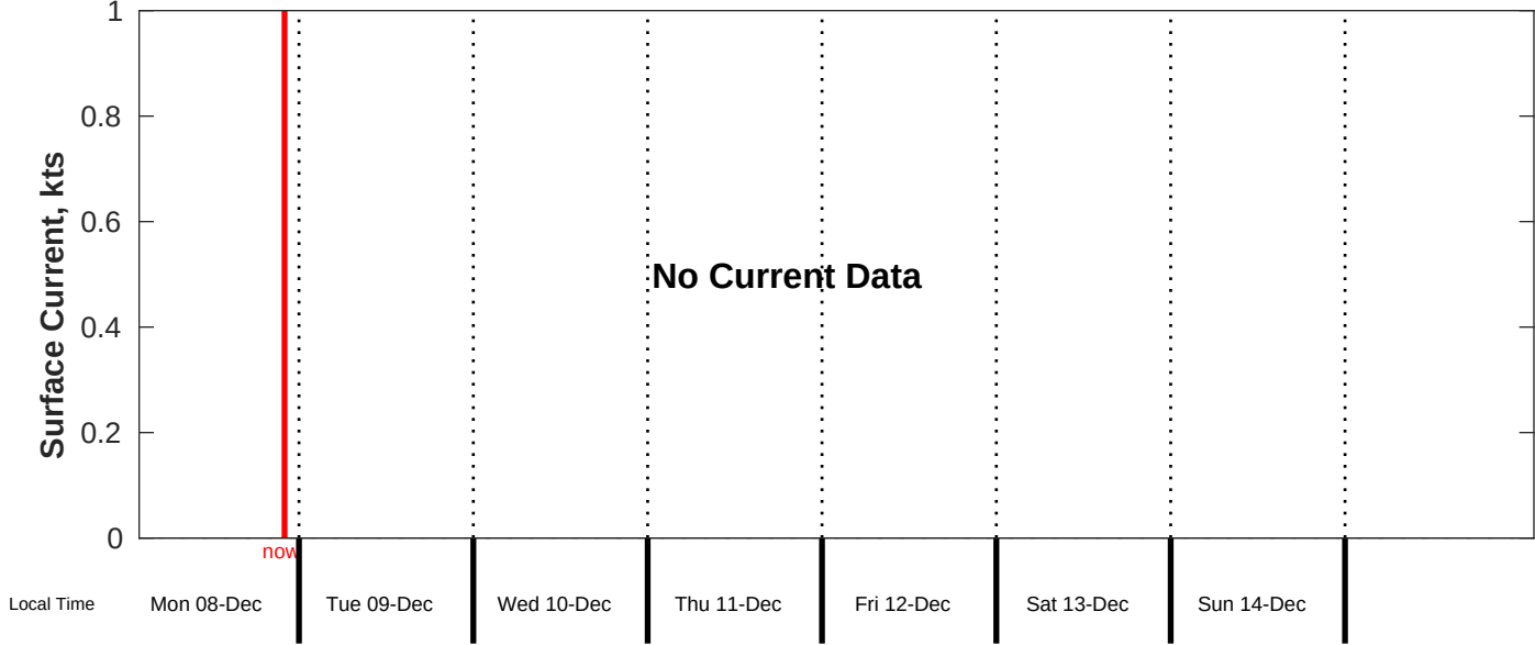
Surface Current Forecast for CSA (ONHYM) PPL EBS - Cote d'Ivoire from 08-Dec-2025 00:00:00 to 16-Dec-2025 00:00:00
