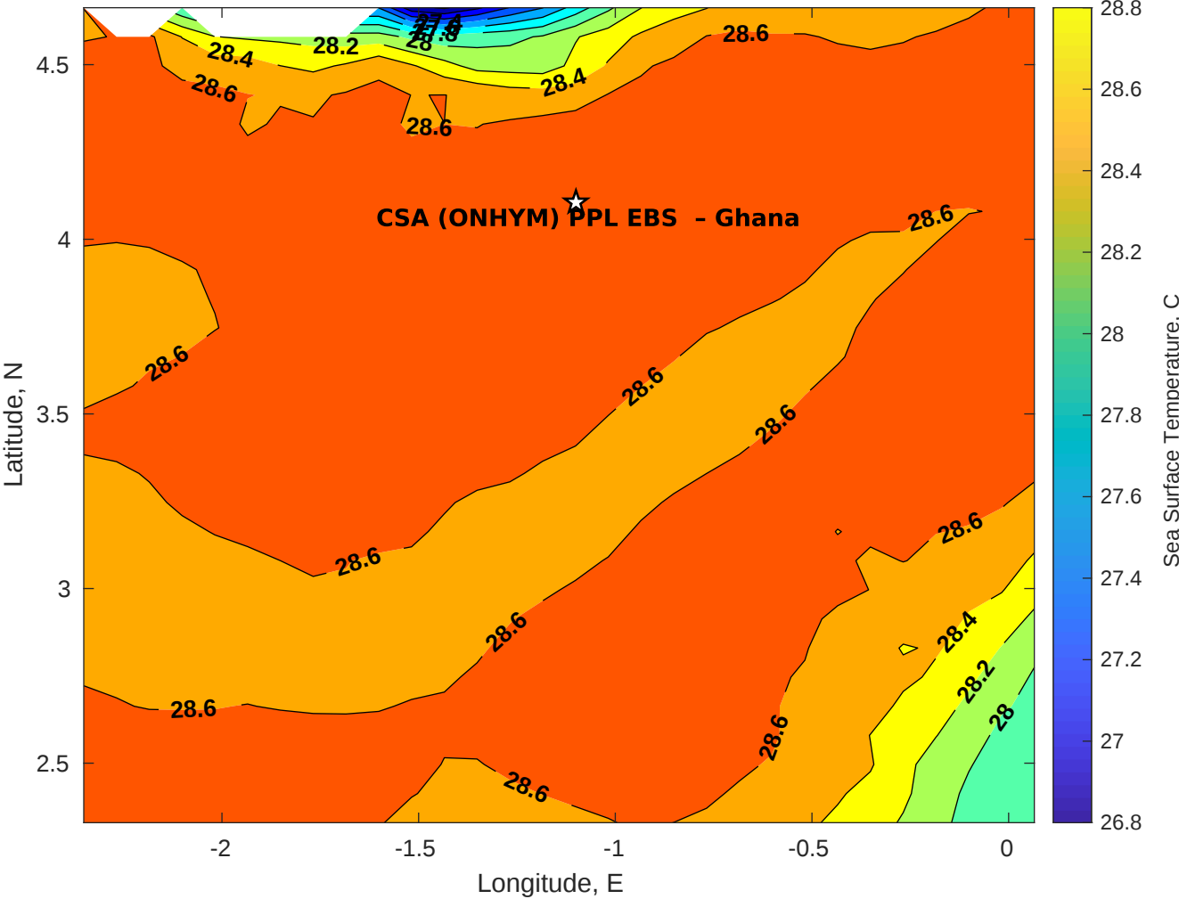
SST for CSA (ONHYM) PPL EBS - Ghana at 08-Dec-2025 00:00:00
