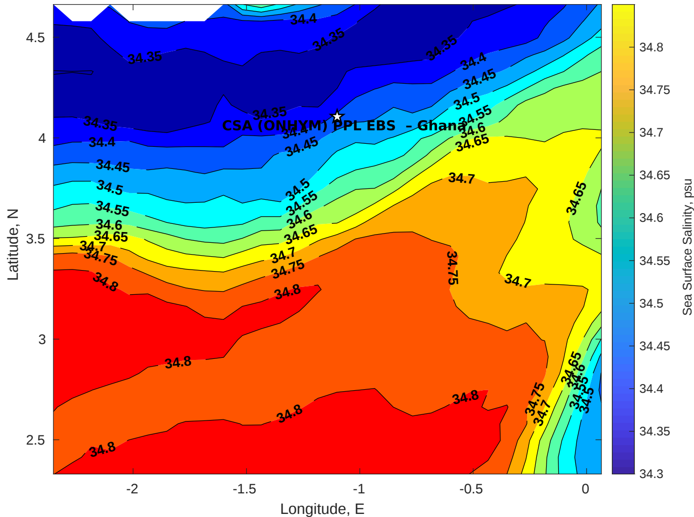
Surface Salinity for CSA (ONHYM) PPL EBS - Ghana at 08-Dec-2025 00:00:00
