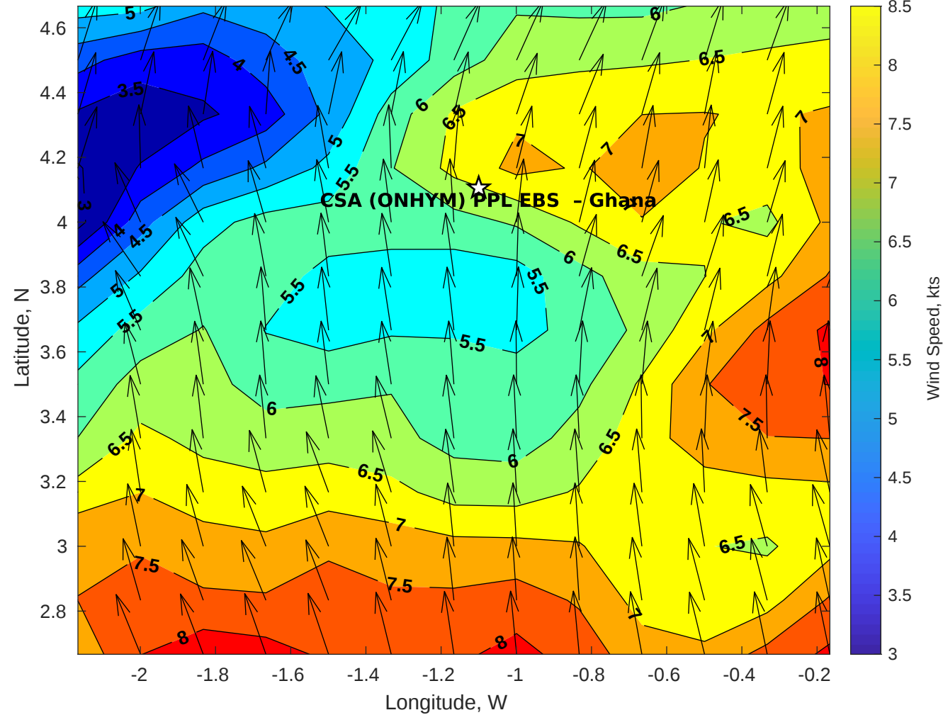
GFS Winds (kts) for CSA (ONHYM) PPL EBS - Ghana at 09-Dec-2025 09:00:00
