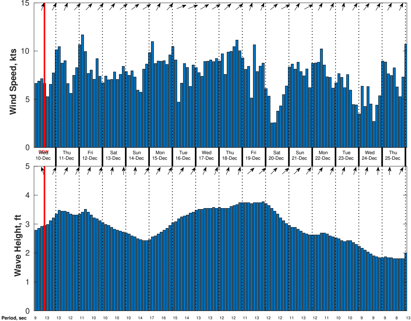
Wind & Wave Forecast for CSA (ONHYM) PPL EBS - Ghana from 09-Dec-2025 02:00:00 to 25-Dec-2025 02:00:00
