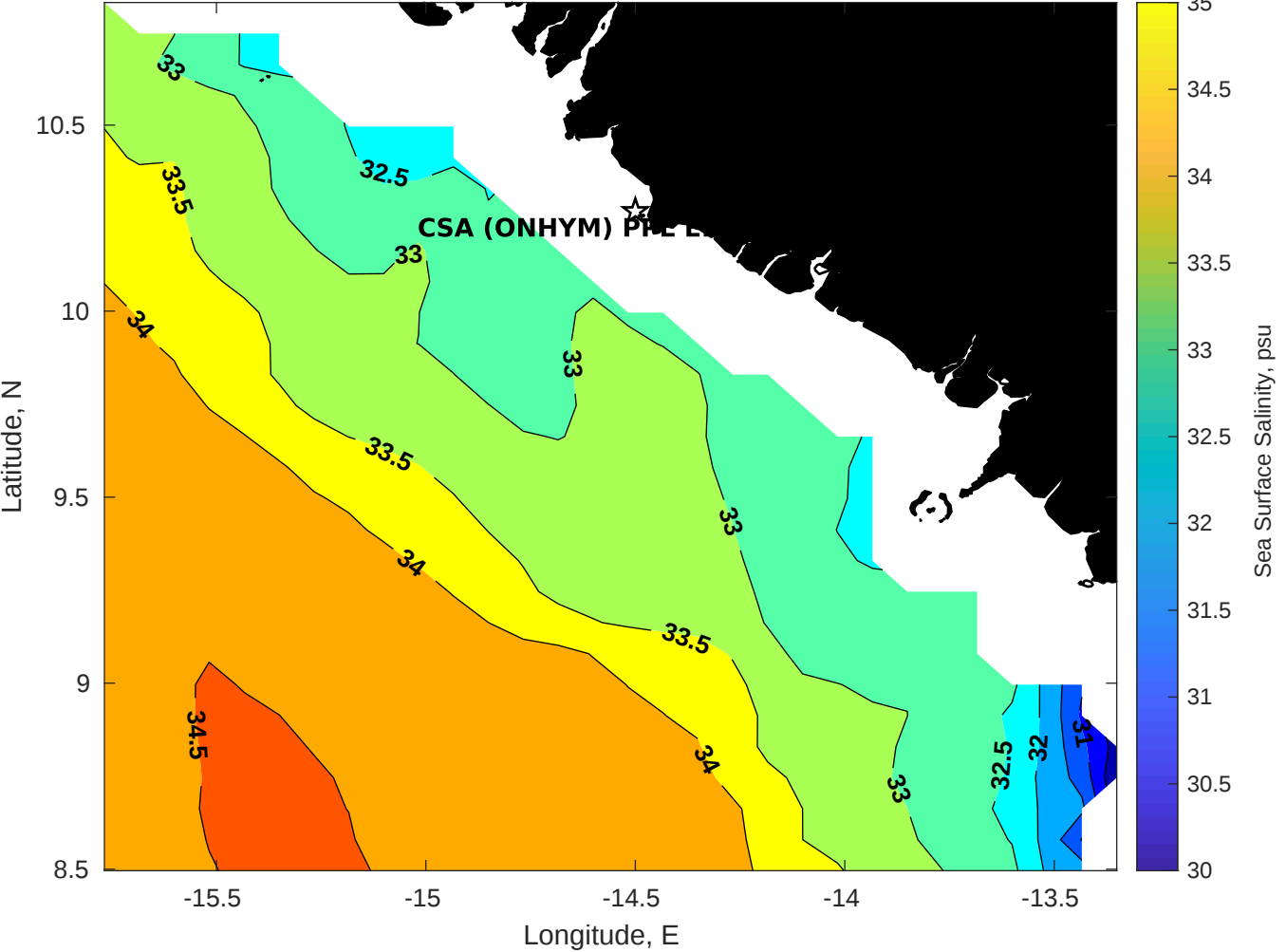
Surface Salinity for CSA (ONHYM) PPL EBS - Guinea at 08-Dec-2025 00:00:00
