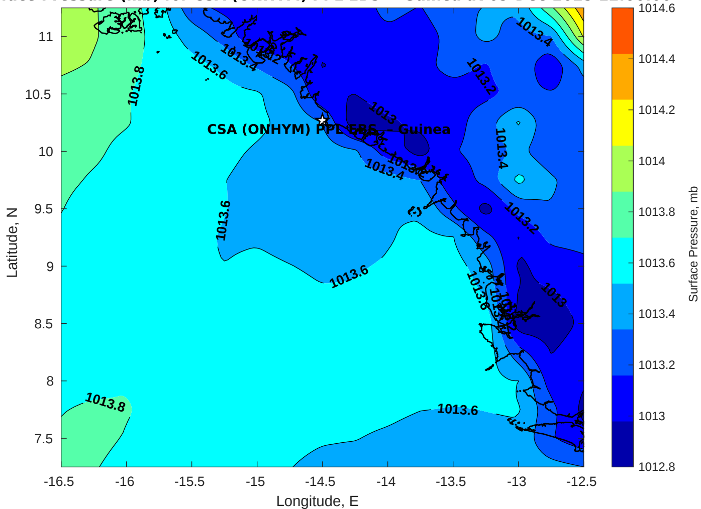
Surface Pressure (mb) for CSA (ONHYM) PPL EBS - Guinea at 09-Dec-2025 12:00:00
