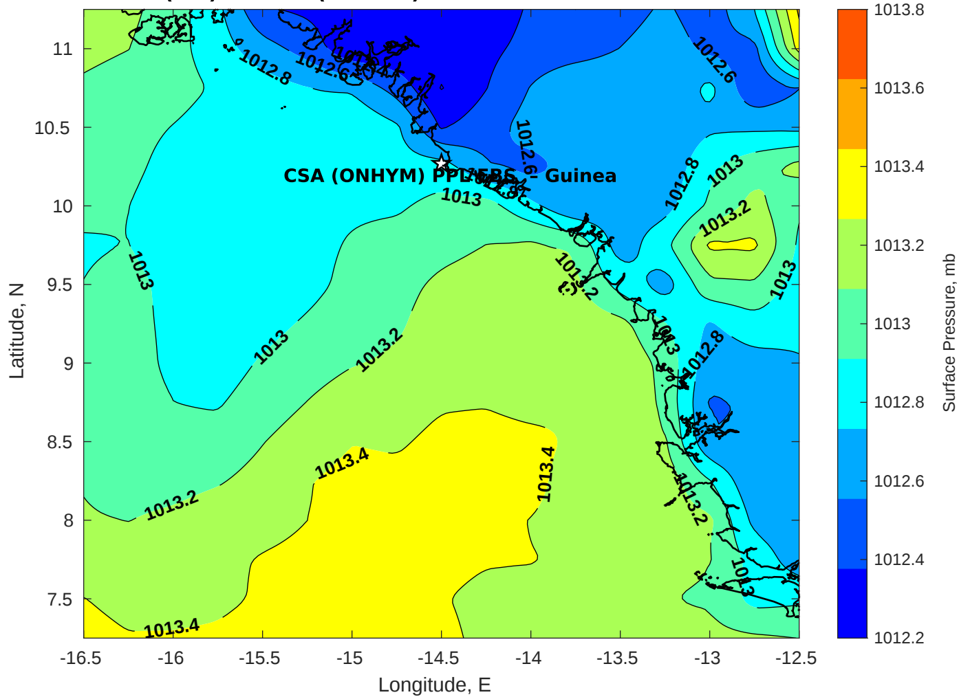
Surface Pressure (mb) for CSA (ONHYM) PPL EBS - Guinea at 10-Dec-2025 12:00:00
