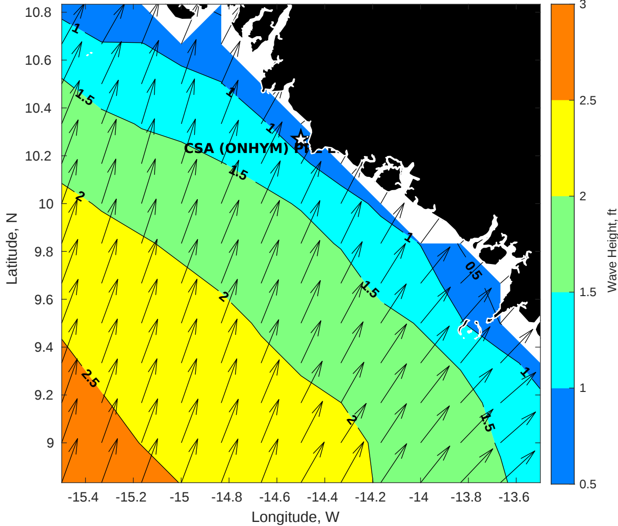
GFS Wave Height (ft) for CSA (ONHYM) PPL EBS - Guinea at 08-Dec-2025 21:00:00
