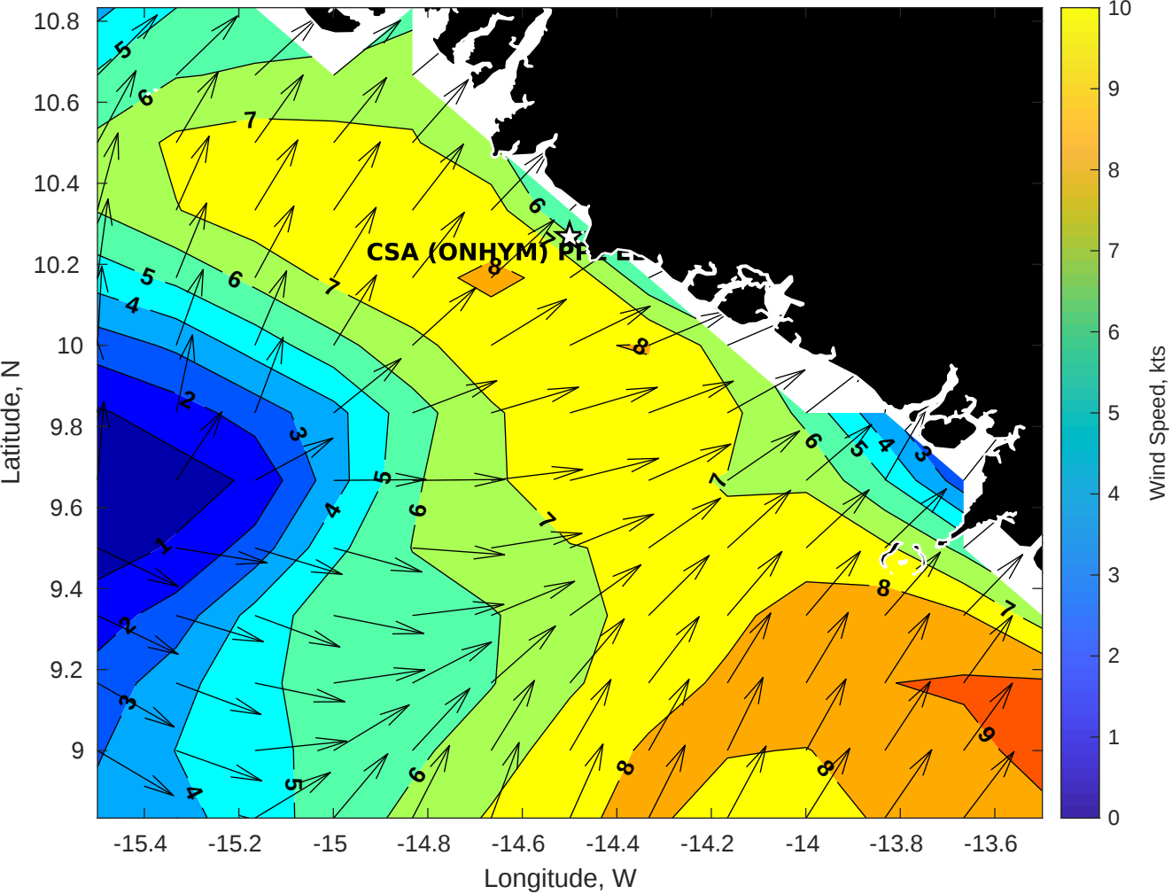
GFS Winds (kts) for CSA (ONHYM) PPL EBS - Guinea at 08-Dec-2025 21:00:00
