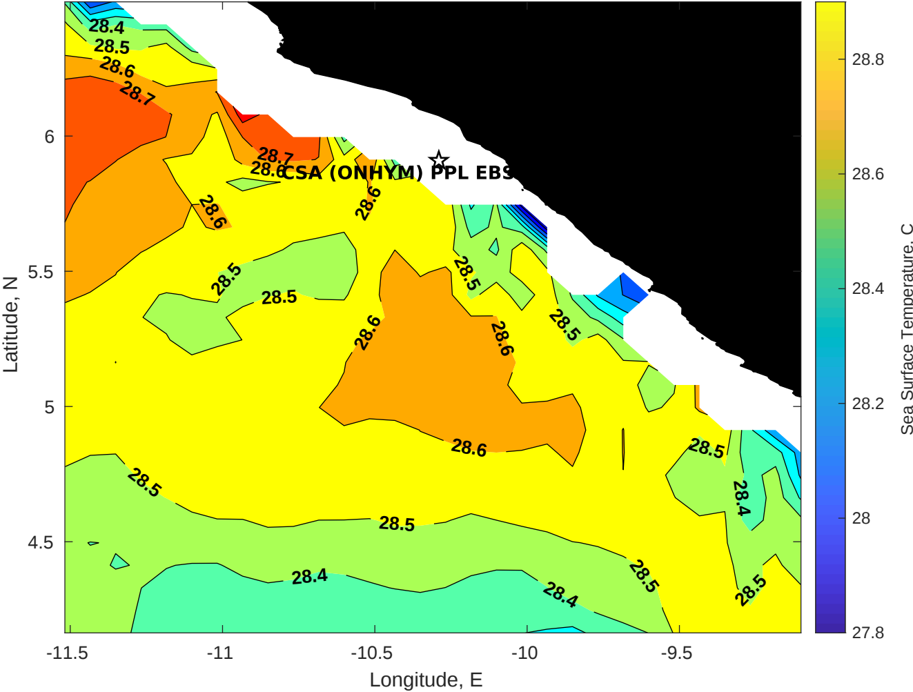
SST for CSA (ONHYM) PPL EBS - Liberia at 08-Dec-2025 00:00:00
