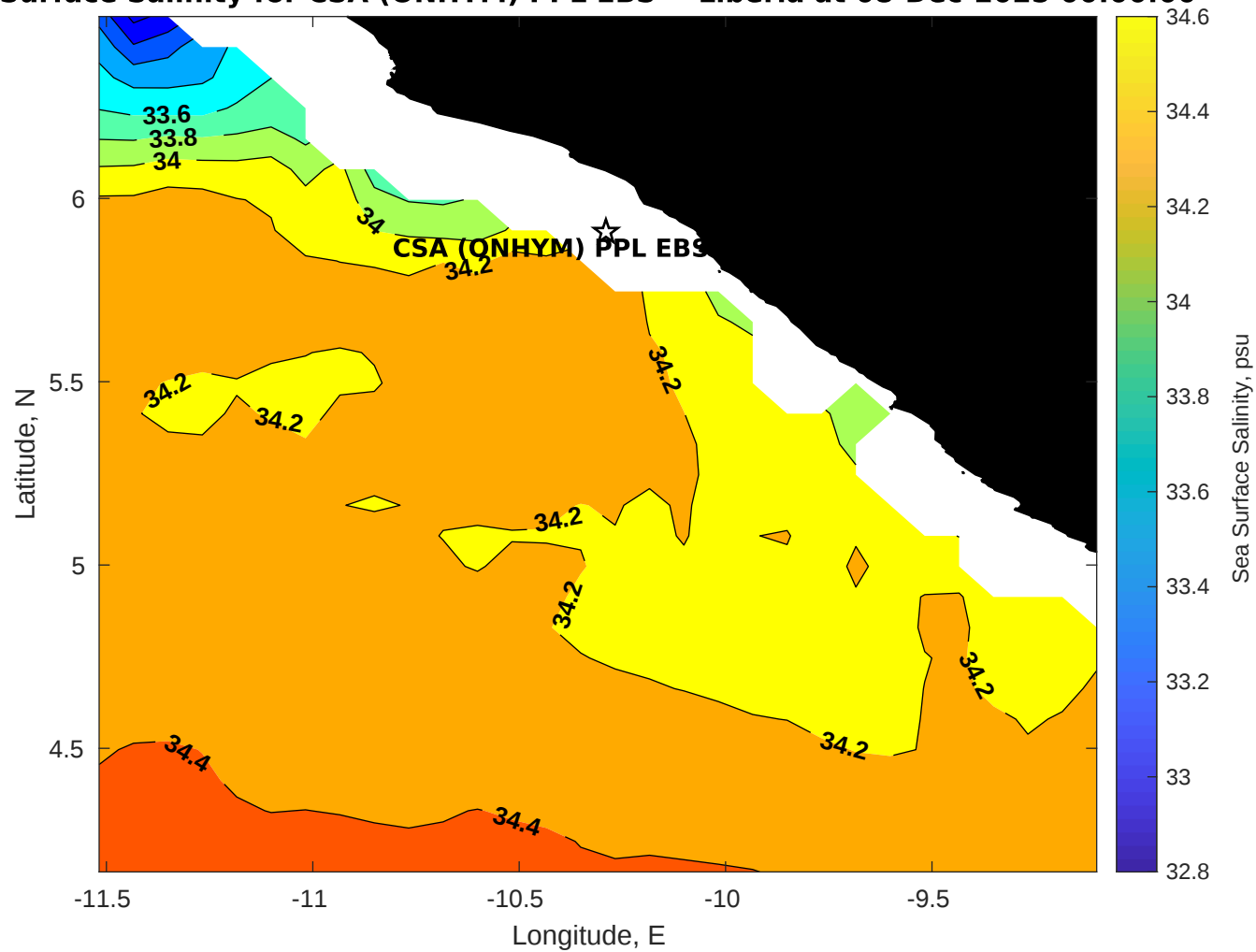
Surface Salinity for CSA (ONHYM) PPL EBS - Liberia at 08-Dec-2025 00:00:00
