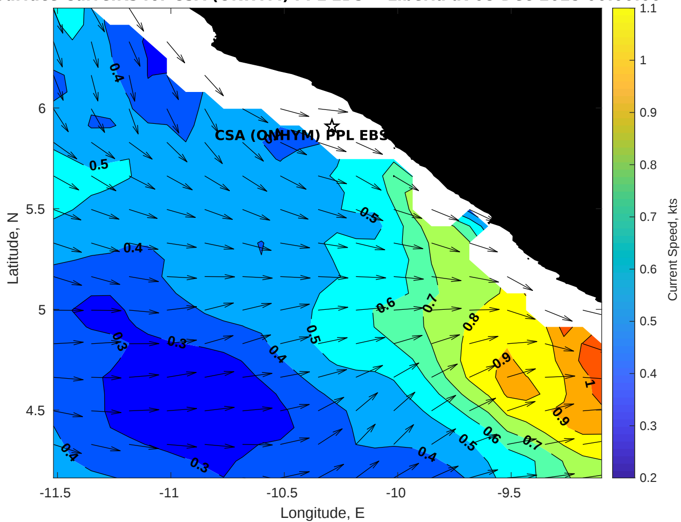
Surface Currents for CSA (ONHYM) PPL EBS - Liberia at 08-Dec-2025 00:00:00
