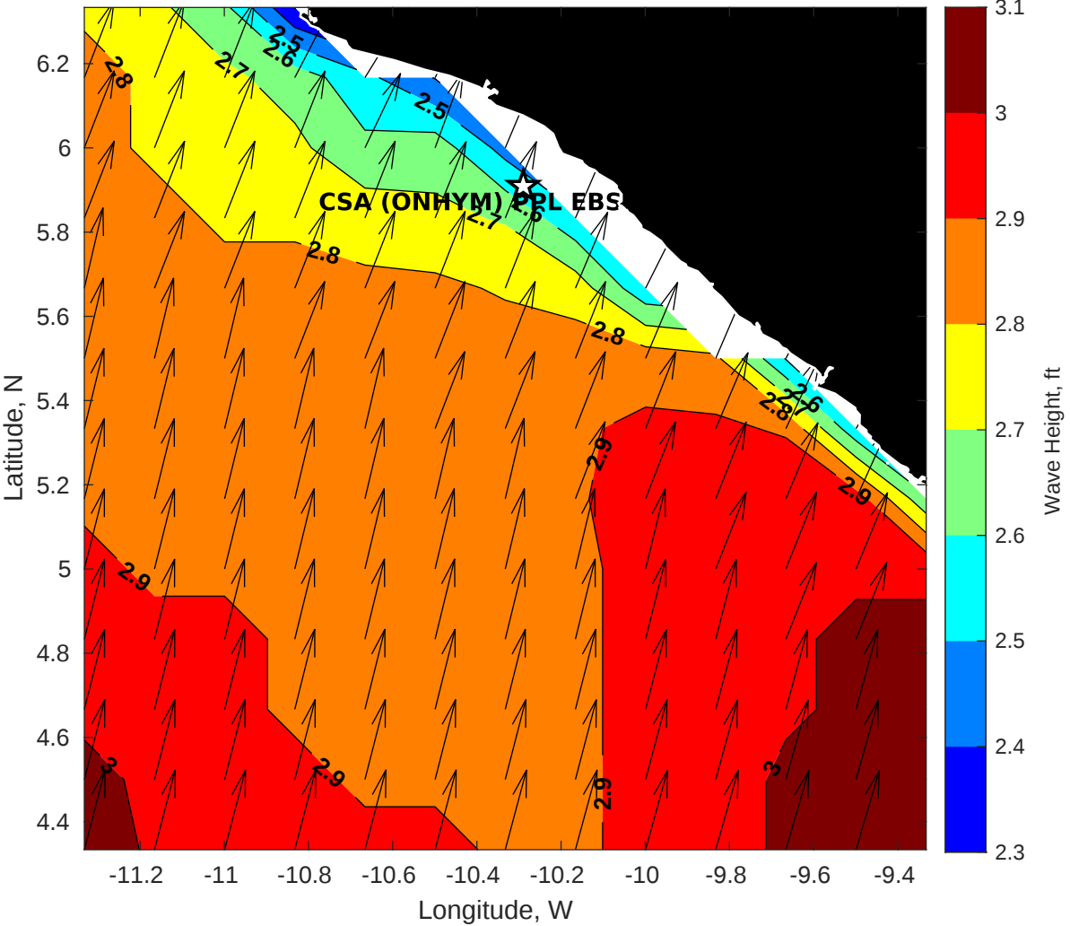
GFS Wave Height (ft) for CSA (ONHYM) PPL EBS - Liberia at 08-Dec-2025 21:00:00
