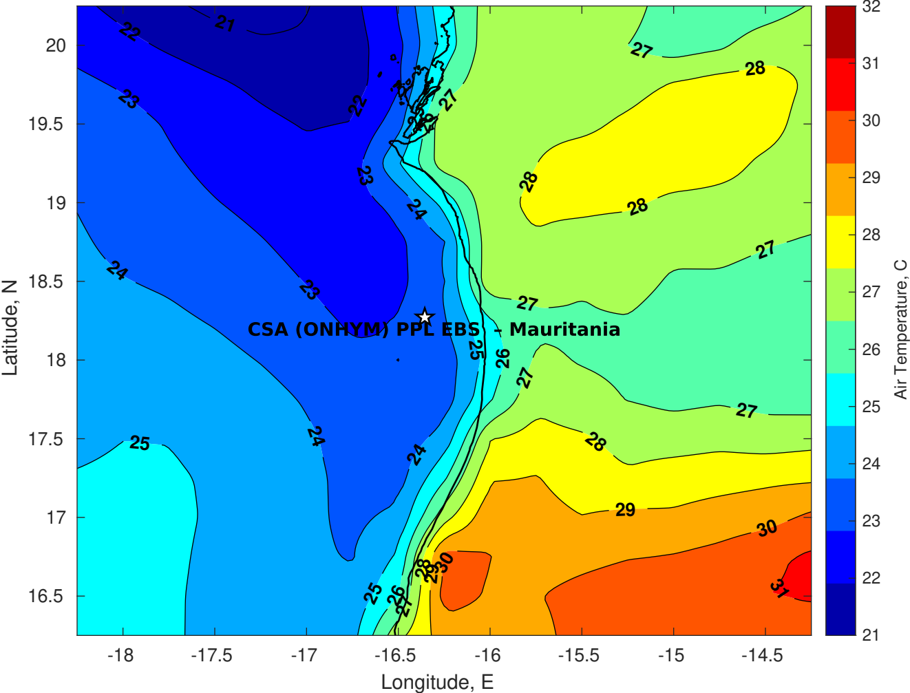
Air Temperature (C) for CSA (ONHYM) PPL EBS - Mauritania at 08-Dec-2025
