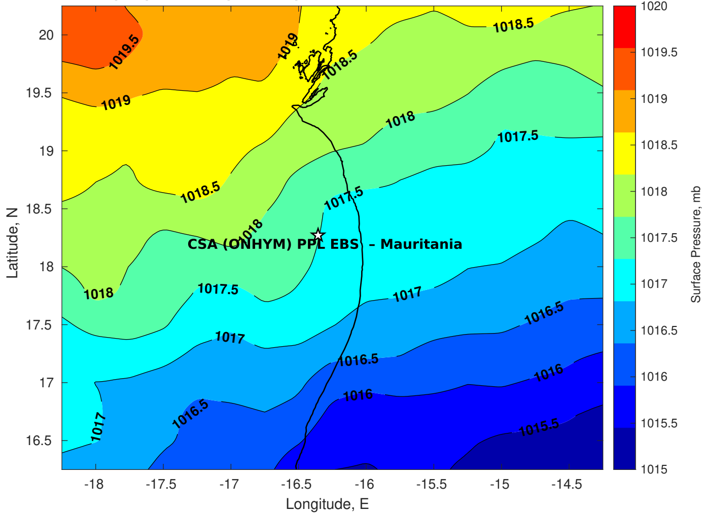
Surface Pressure (mb) for CSA (ONHYM) PPL EBS - Mauritania at 10-Dec-2025 12:00:00
