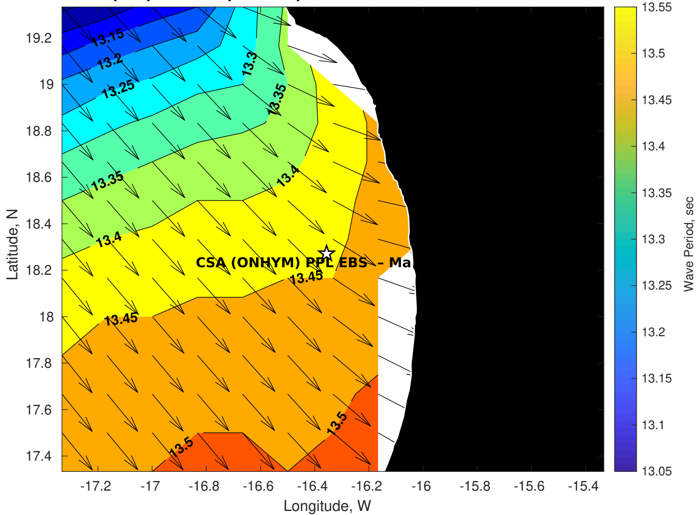
GFS Wave Period (sec) for CSA (ONHYM) PPL EBS - Mauritania at 08-Dec-2025 21:00:00
