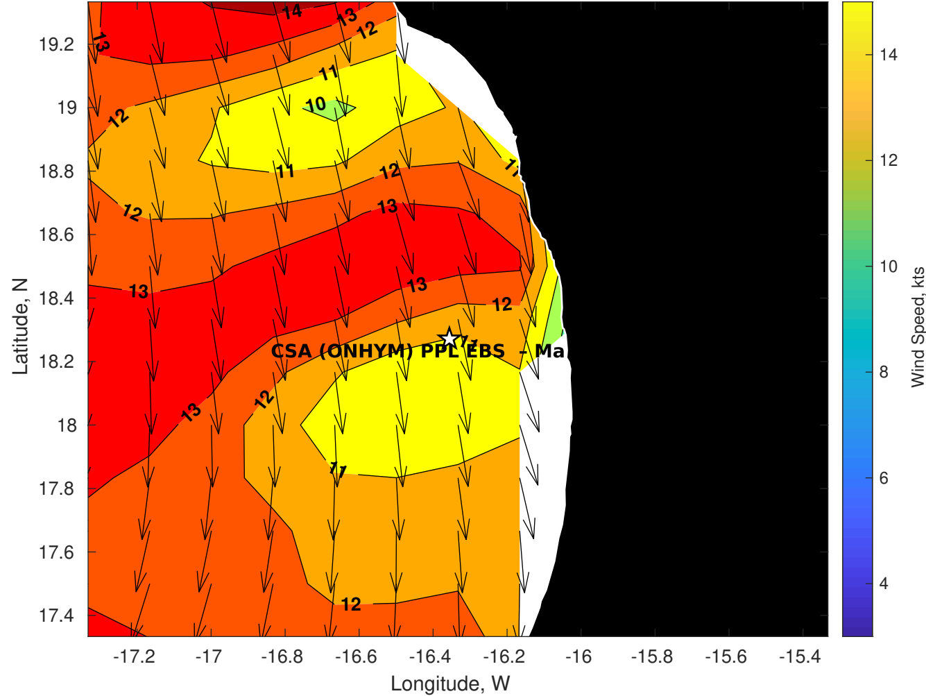
GFS Winds (kts) for CSA (ONHYM) PPL EBS - Mauritania at 08-Dec-2025 21:00:00
