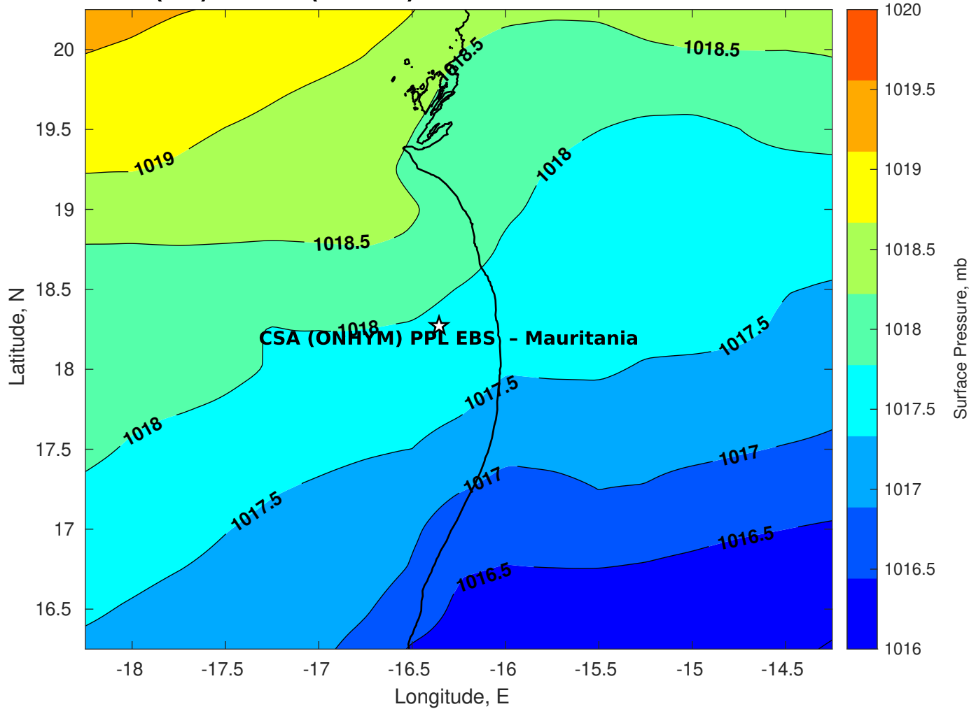
Surface Pressure (mb) for CSA (ONHYM) PPL EBS - Mauritania at 09-Dec-2025 12:00:00
