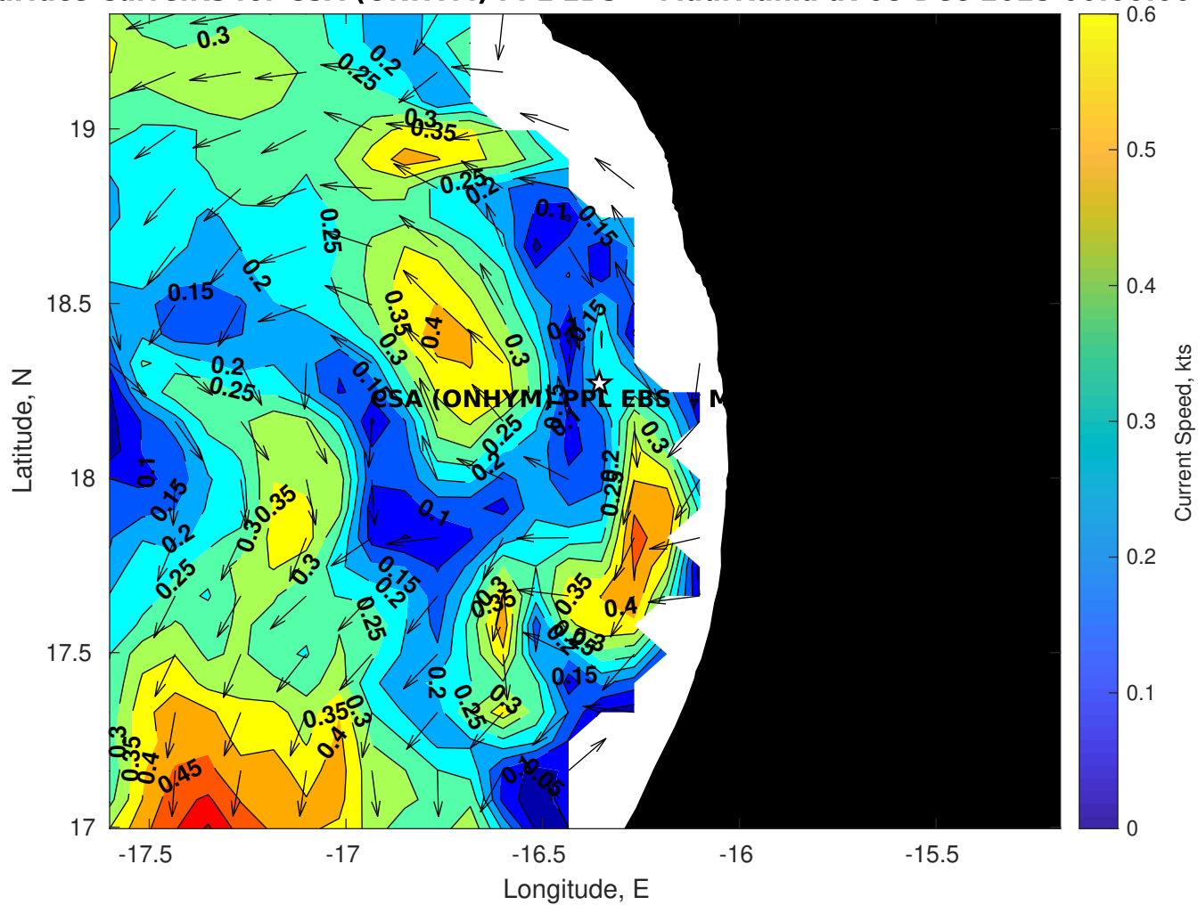
Surface Currents for CSA (ONHYM) PPL EBS - Mauritania at 08-Dec-2025 00:00:00
