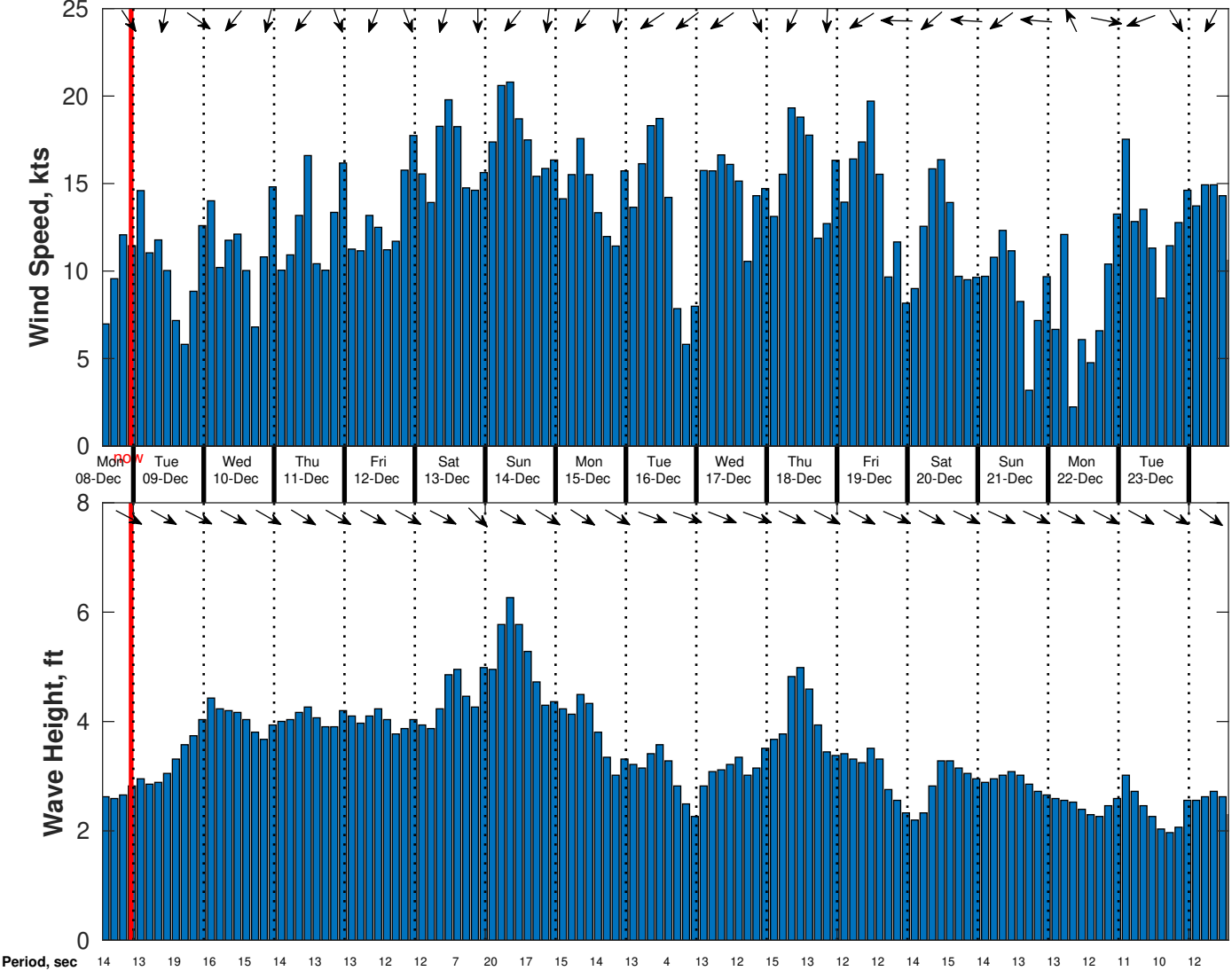
Wind & Wave Forecast for CSA (ONHYM) PPL EBS - Mauritania from 08-Dec-2025 13:00:00 to 24-Dec-2025 13:00:00
