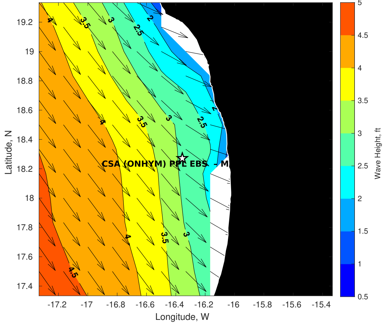
GFS Wave Height (ft) for CSA (ONHYM) PPL EBS - Mauritania at 08-Dec-2025 21:00:00
