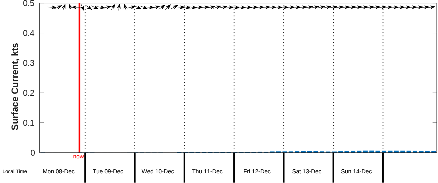
Surface Current Forecast for CSA (ONHYM) PPL EBS - Mauritania from 08-Dec-2025 00:00:00 to 16-Dec-2025 00:00:00
