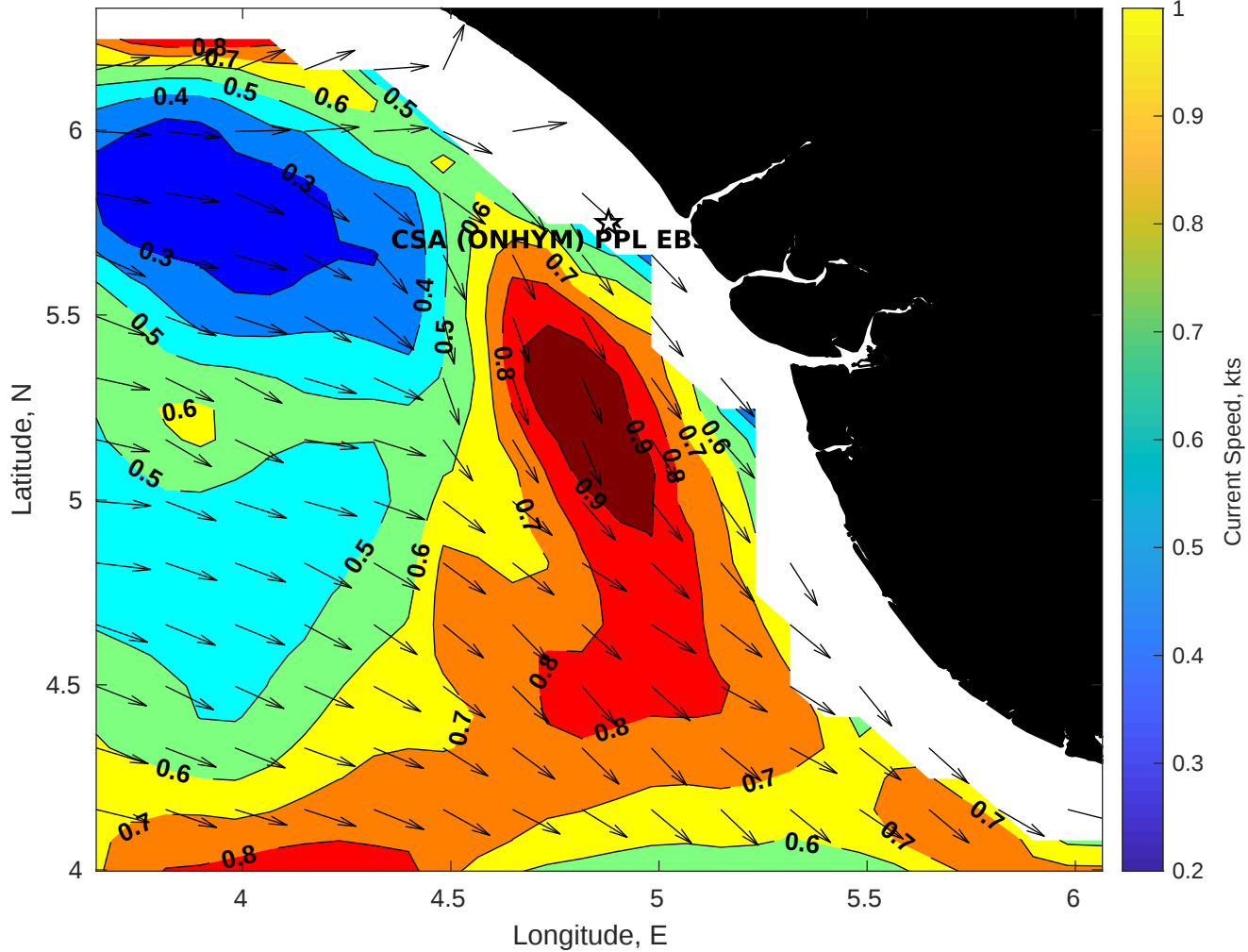
Surface Currents for CSA (ONHYM) PPL EBS - Nigeria at 08-Dec-2025 00:00:00
