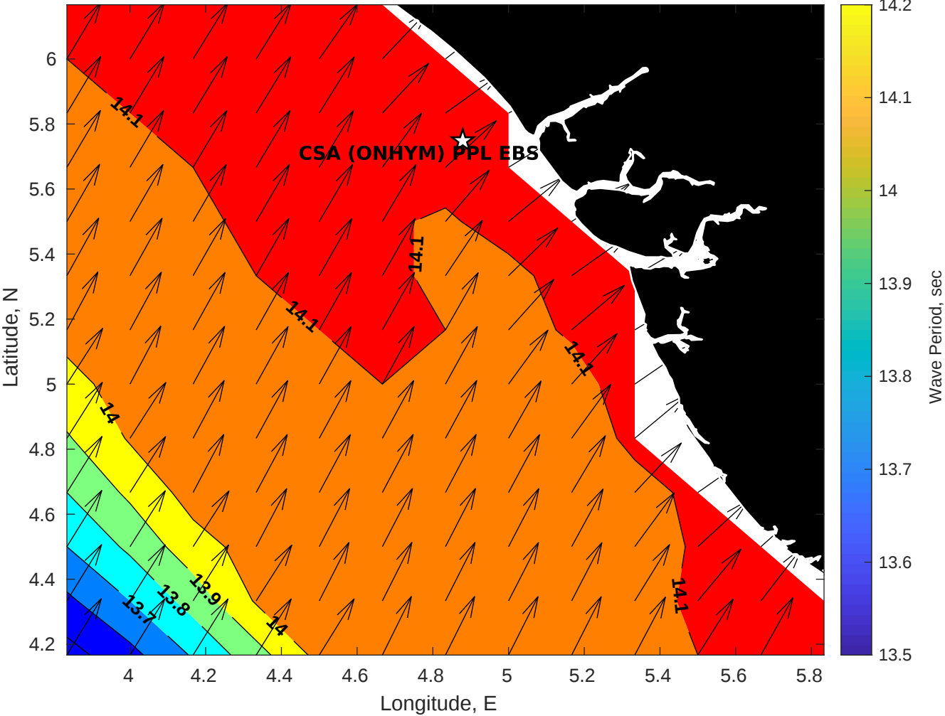
GFS Wave Period (sec) for CSA (ONHYM) PPL EBS - Nigeria at 09-Dec-2025 09:00:00
