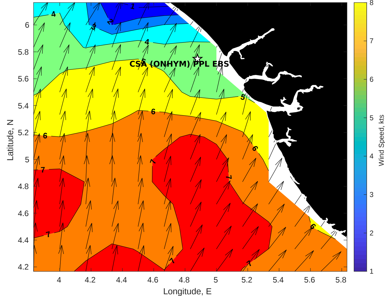
GFS Winds (kts) for CSA (ONHYM) PPL EBS - Nigeria at 09-Dec-2025 09:00:00
