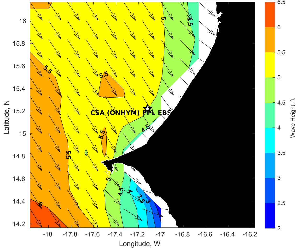
GFS Wave Height (ft) for CSA (ONHYM) PPL EBS - Senegal at 08-Dec-2025 21:00:00
