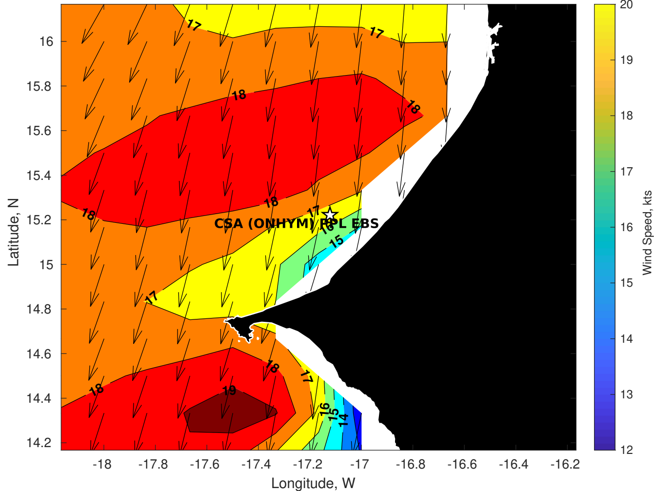
GFS Winds (kts) for CSA (ONHYM) PPL EBS - Senegal at 08-Dec-2025 21:00:00
