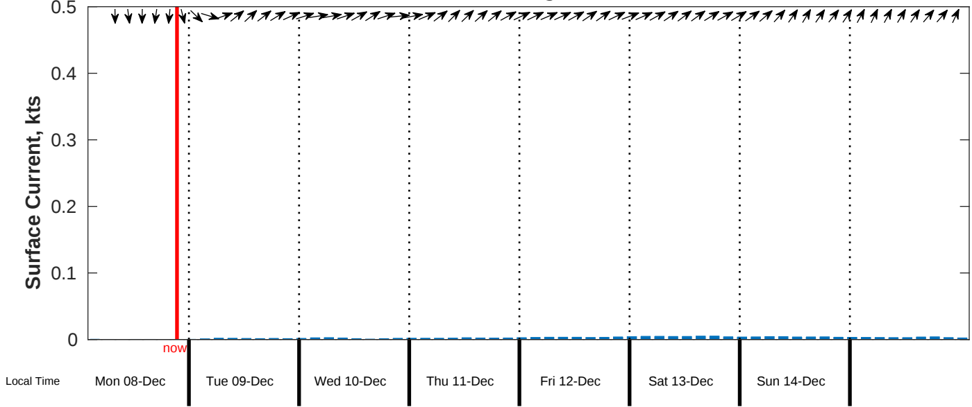
Surface Current Forecast for CSA (ONHYM) PPL EBS - Senegal from 08-Dec-2025 00:00:00 to 16-Dec-2025 00:00:00
