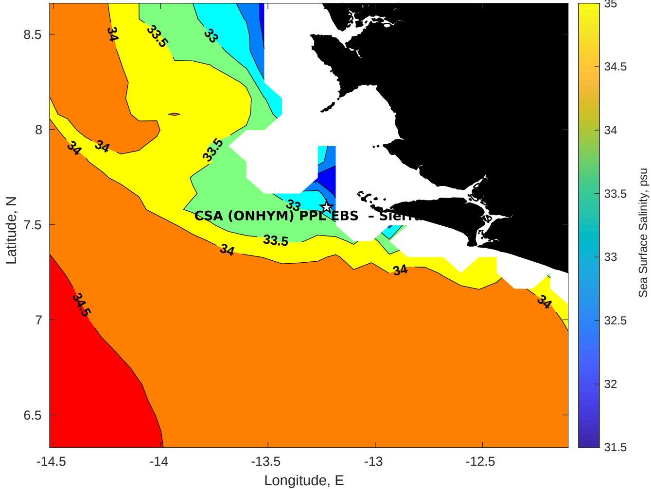
Surface Salinity for CSA (ONHYM) PPL EBS - Sierra Leone at 08-Dec-2025 00:00:00
