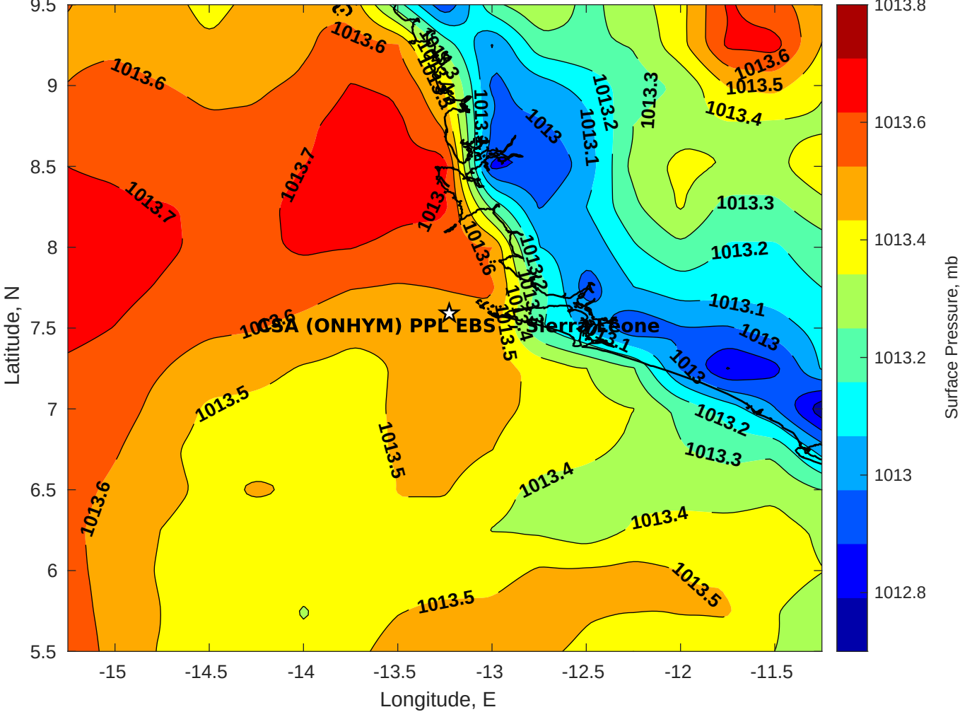
Surface Pressure (mb) for CSA (ONHYM) PPL EBS - Sierra Leone at 09-Dec-2025 12:00:00
